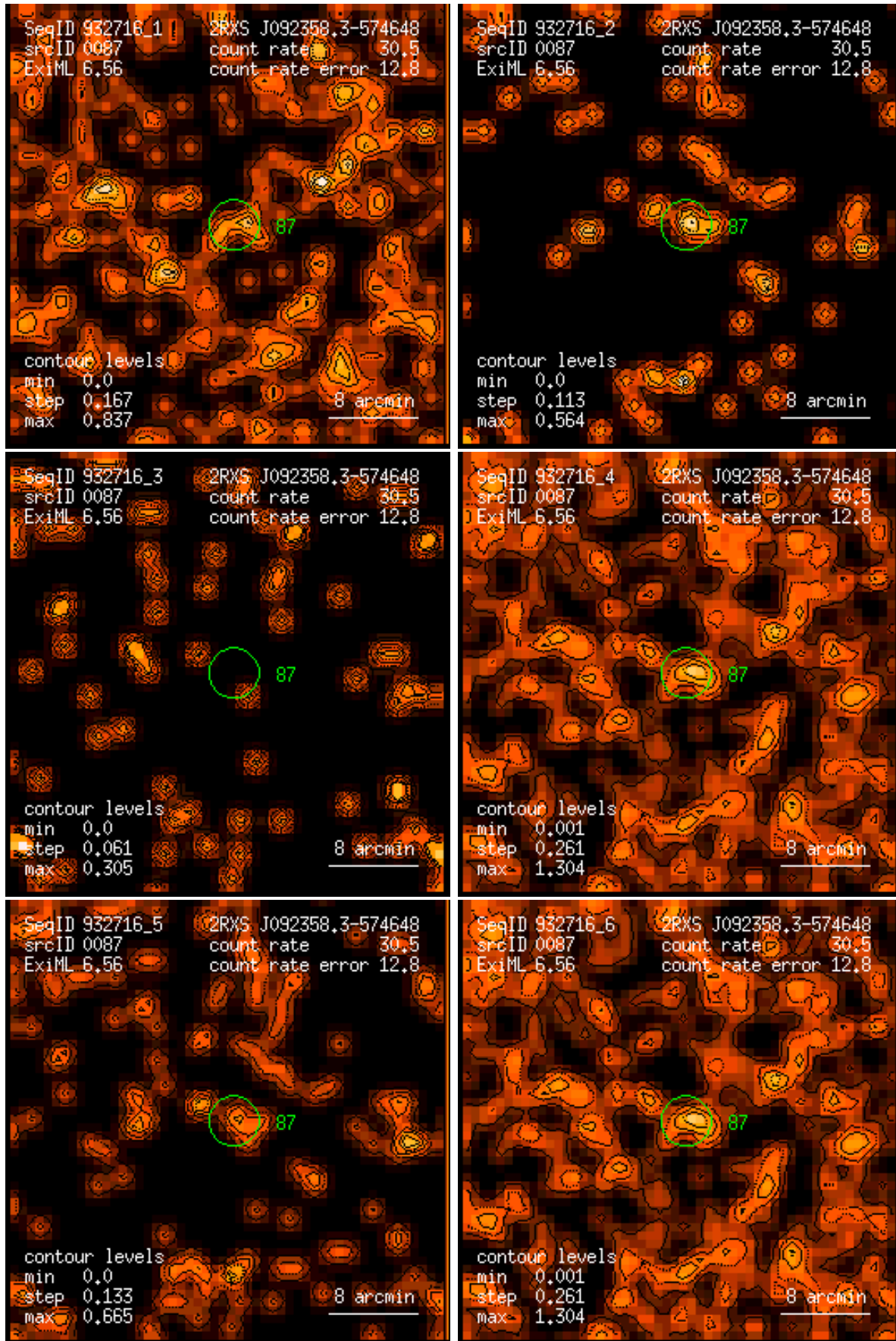
Figure 87: RASS 932716: detection 0087: band rate images, Gaussian filter: (1) PSPC channels 11 – 41, (2) 52 – 90, (3) 91 – 201, (4) 11 – 235, (5) 52 – 201, (6) 11 – 201. Broad band rates in counts/ks. Band rate contour levels in counts/ks/arcmin 2 .
