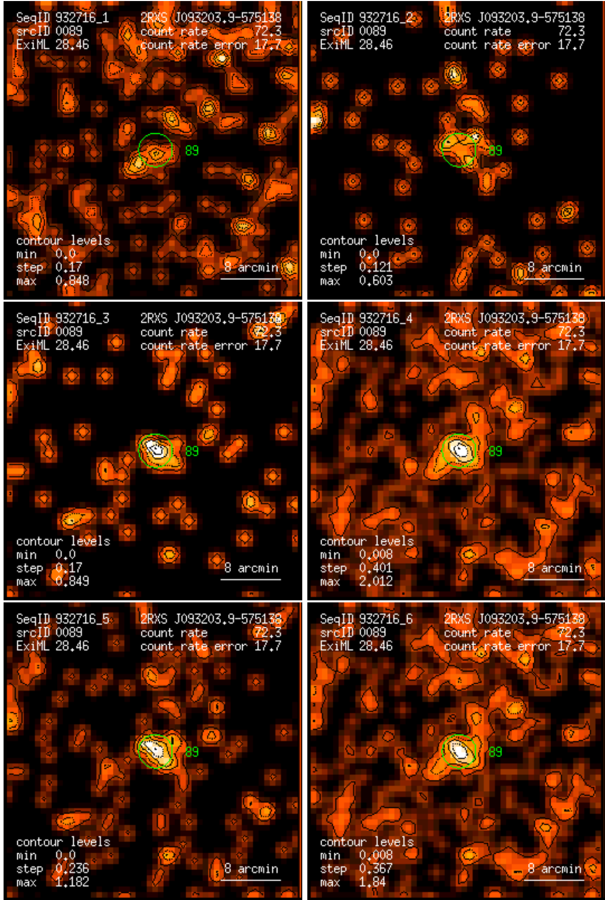
Figure 89: RASS 932716: detection 0089: band rate images, Gaussian filter: (1) PSPC channels 11 – 41, (2) 52 – 90, (3) 91 – 201, (4) 11 – 235, (5) 52 – 201, (6) 11 – 201. Broad band rates in counts/ks. Band rate contour levels in counts/ks/arcmin 2 .
