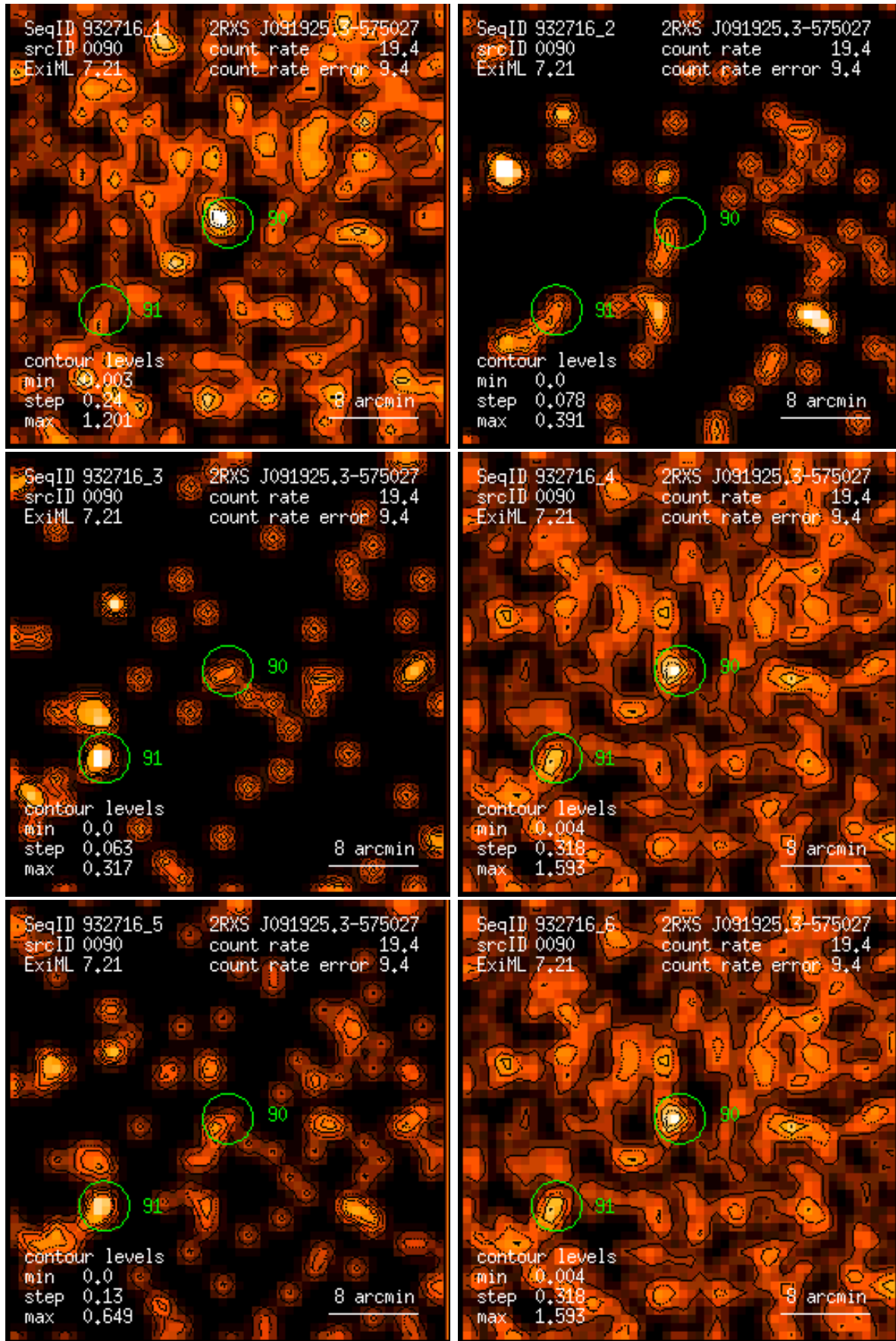
Figure 90: RASS 932716: detection 0090: band rate images, Gaussian filter: (1) PSPC channels 11 – 41, (2) 52 – 90, (3) 91 – 201, (4) 11 – 235, (5) 52 – 201, (6) 11 – 201. Broad band rates in counts/ks. Band rate contour levels in counts/ks/arcmin 2 .
