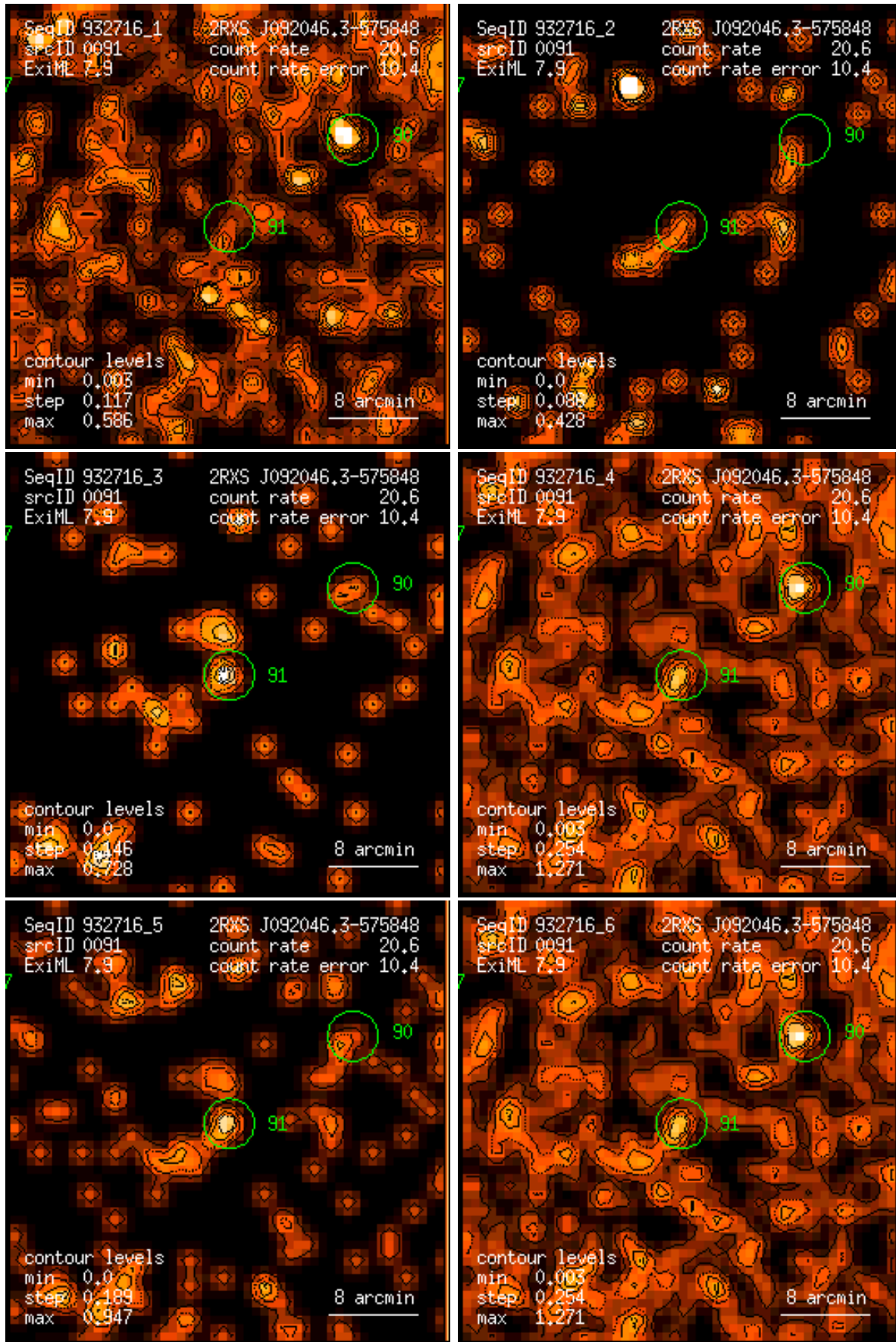
Figure 91: RASS 932716: detection 0091: band rate images, Gaussian filter: (1) PSPC channels 11 – 41, (2) 52 – 90, (3) 91 – 201, (4) 11 – 235, (5) 52 – 201, (6) 11 – 201. Broad band rates in counts/ks. Band rate contour levels in counts/ks/arcmin 2 .
