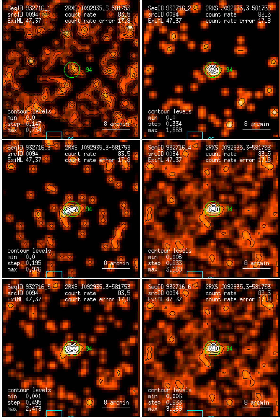
Figure 94: RASS 932716: detection 0094: band rate images, Gaussian filter: (1) PSPC channels 11 – 41, (2) 52 – 90, (3) 91 – 201, (4) 11 – 235, (5) 52 – 201, (6) 11 – 201. Broad band rates in counts/ks. Band rate contour levels in counts/ks/arcmin 2 .
