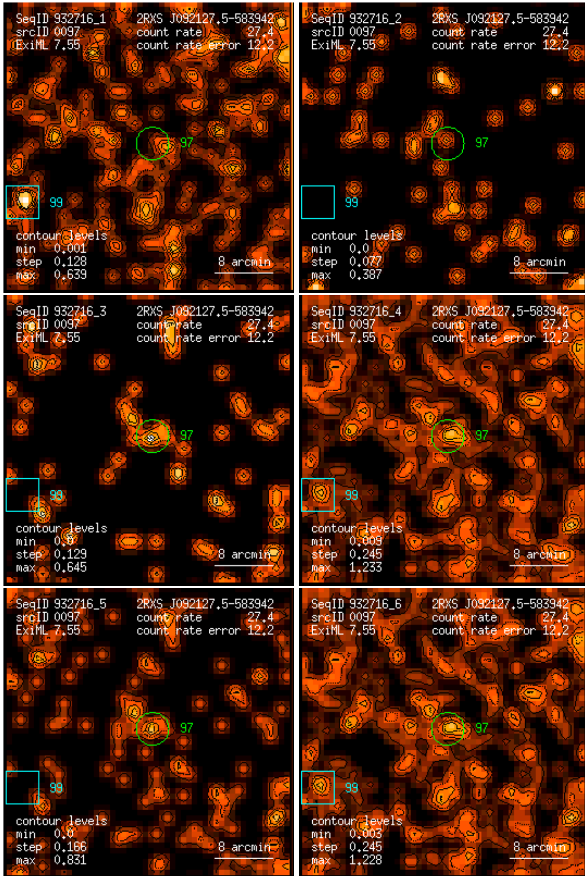
Figure 97: RASS 932716: detection 0097: band rate images, Gaussian filter: (1) PSPC channels 11 – 41, (2) 52 – 90, (3) 91 – 201, (4) 11 – 235, (5) 52 – 201, (6) 11 – 201. Broad band rates in counts/ks. Band rate contour levels in counts/ks/arcmin 2 .
