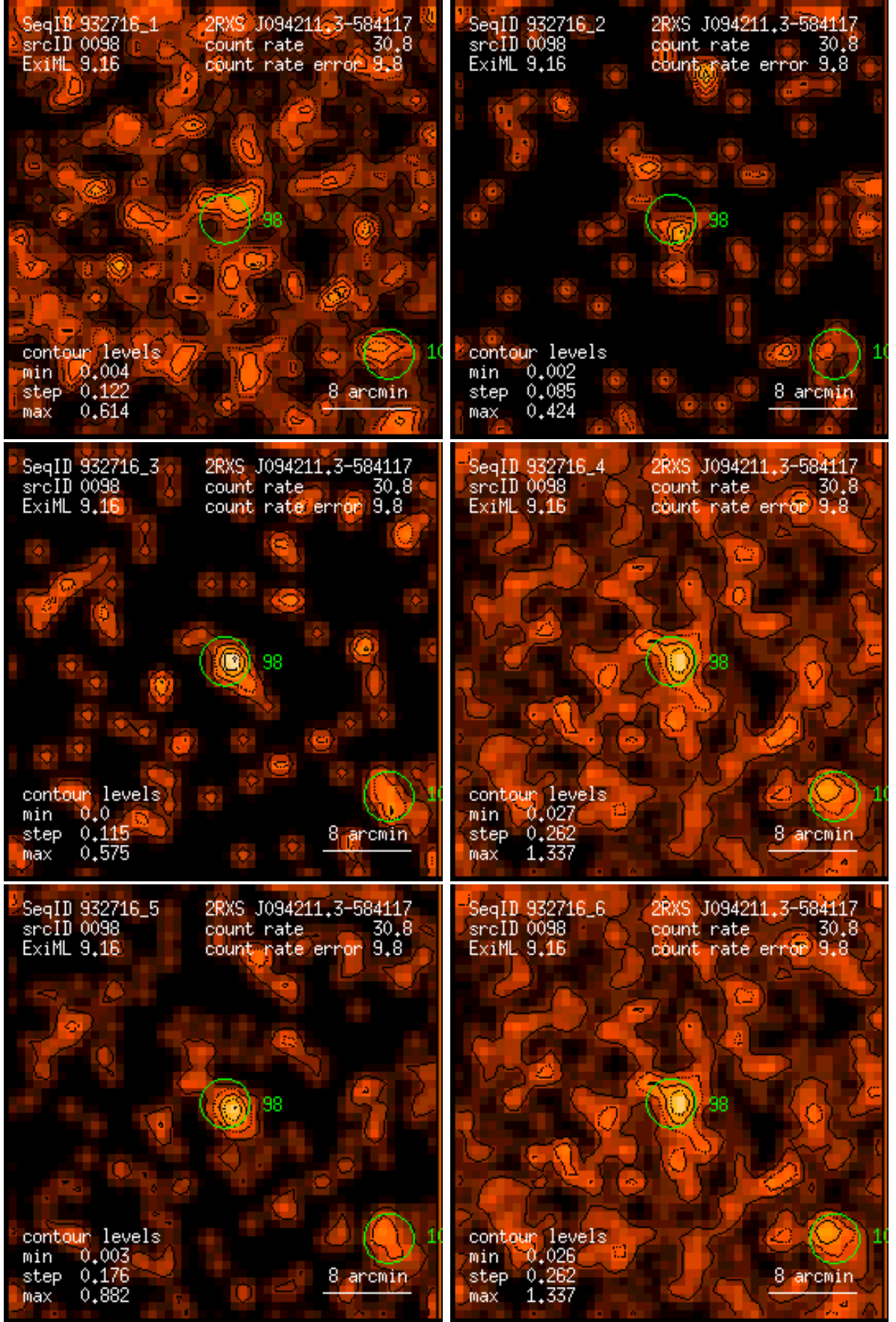
Figure 98: RASS 932716: detection 0098: band rate images, Gaussian filter: (1) PSPC channels 11 – 41, (2) 52 – 90, (3) 91 – 201, (4) 11 – 235, (5) 52 – 201, (6) 11 – 201. Broad band rates in counts/ks. Band rate contour levels in counts/ks/arcmin 2 .
