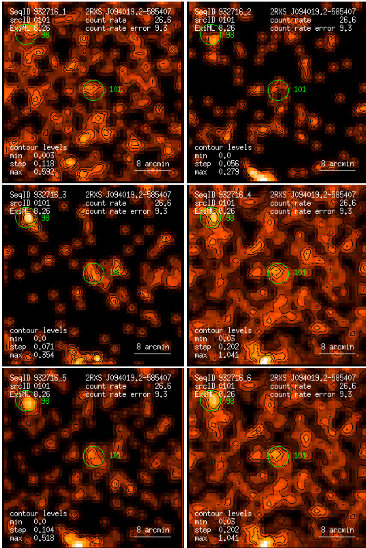
Figure 101: RASS 932716: detection 0101: band rate images, Gaussian filter: (1) PSPC channels 11 – 41, (2) 52 – 90, (3) 91 – 201, (4) 11 – 235, (5) 52 – 201, (6) 11 – 201. Broad band rates in counts/ks. Band rate contour levels in counts/ks/arcmin 2 .
