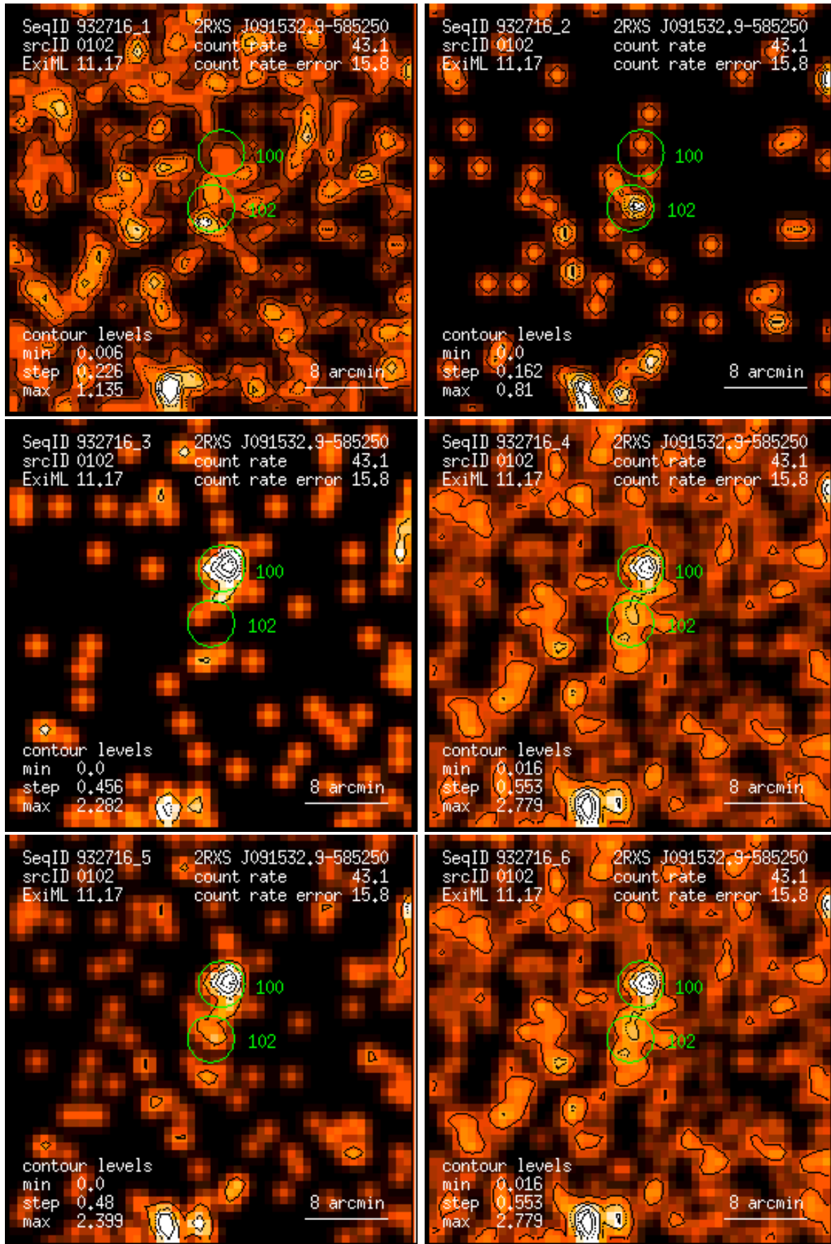
Figure 102: RASS 932716: detection 0102: band rate images, Gaussian filter: (1) PSPC channels 11 – 41, (2) 52 – 90, (3) 91 – 201, (4) 11 – 235, (5) 52 – 201, (6) 11 – 201. Broad band rates in counts/ks. Band rate contour levels in counts/ks/arcmin 2 .
