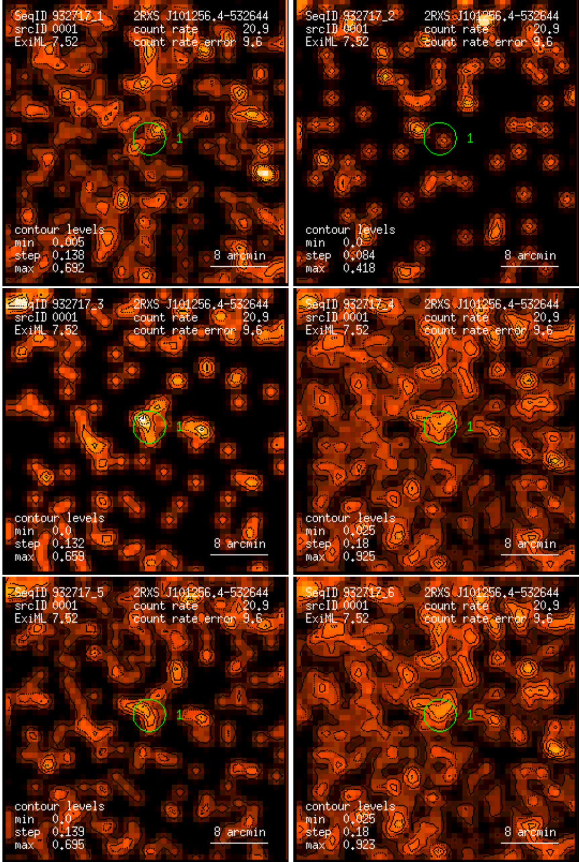
Figure 1: RASS 932717: detection 0001: band rate images, Gaussian filter: (1) PSPC channels 11 – 41, (2) 52 – 90, (3) 91 – 201, (4) 11 – 235, (5) 52 – 201, (6) 11 – 201. Broad band rates in counts/ks. Band rate contour levels in counts/ks/arcmin 2 .
