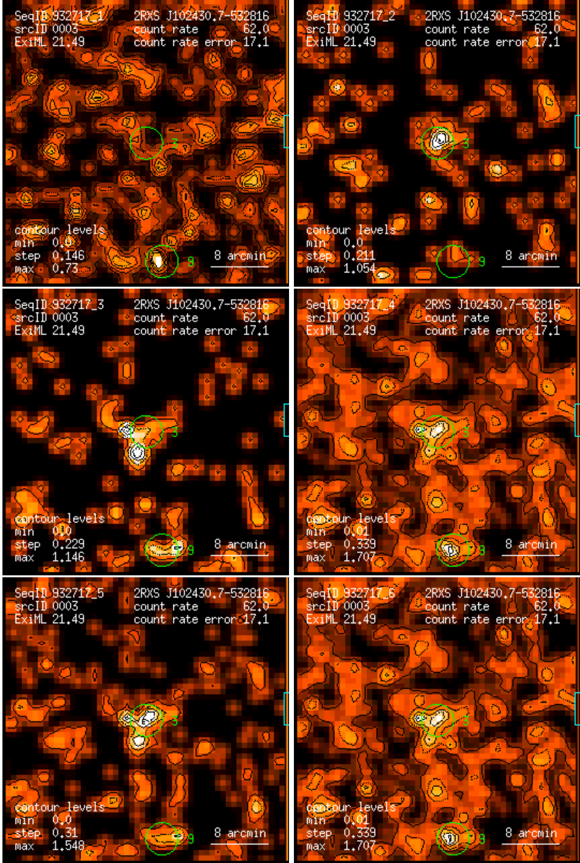
Figure 3: RASS 932717: detection 0003: band rate images, Gaussian filter: (1) PSPC channels 11 – 41, (2) 52 – 90, (3) 91 – 201, (4) 11 – 235, (5) 52 – 201, (6) 11 – 201. Broad band rates in counts/ks. Band rate contour levels in counts/ks/arcmin 2 .
