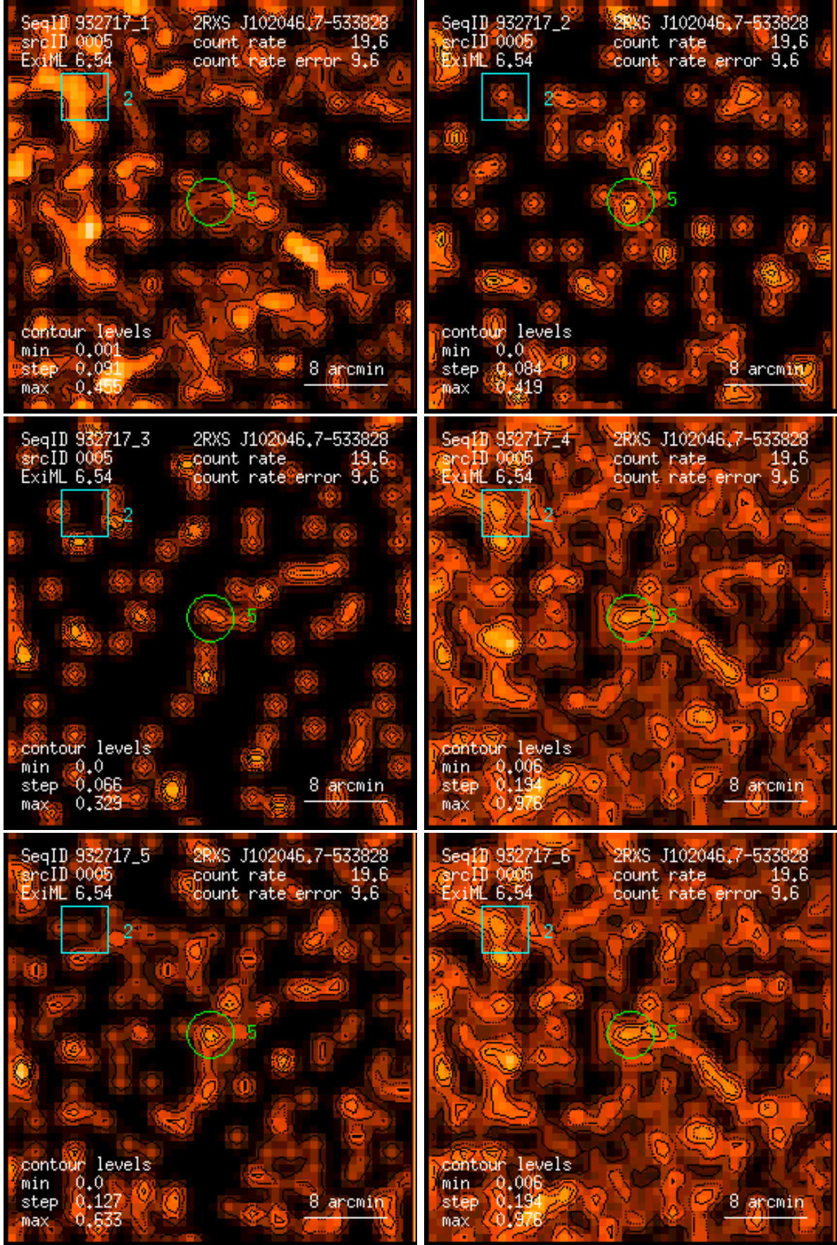
Figure 5: RASS 932717: detection 0005: band rate images, Gaussian filter: (1) PSPC channels 11 – 41, (2) 52 – 90, (3) 91 – 201, (4) 11 – 235, (5) 52 – 201, (6) 11 – 201. Broad band rates in counts/ks. Band rate contour levels in counts/ks/arcmin 2 .
