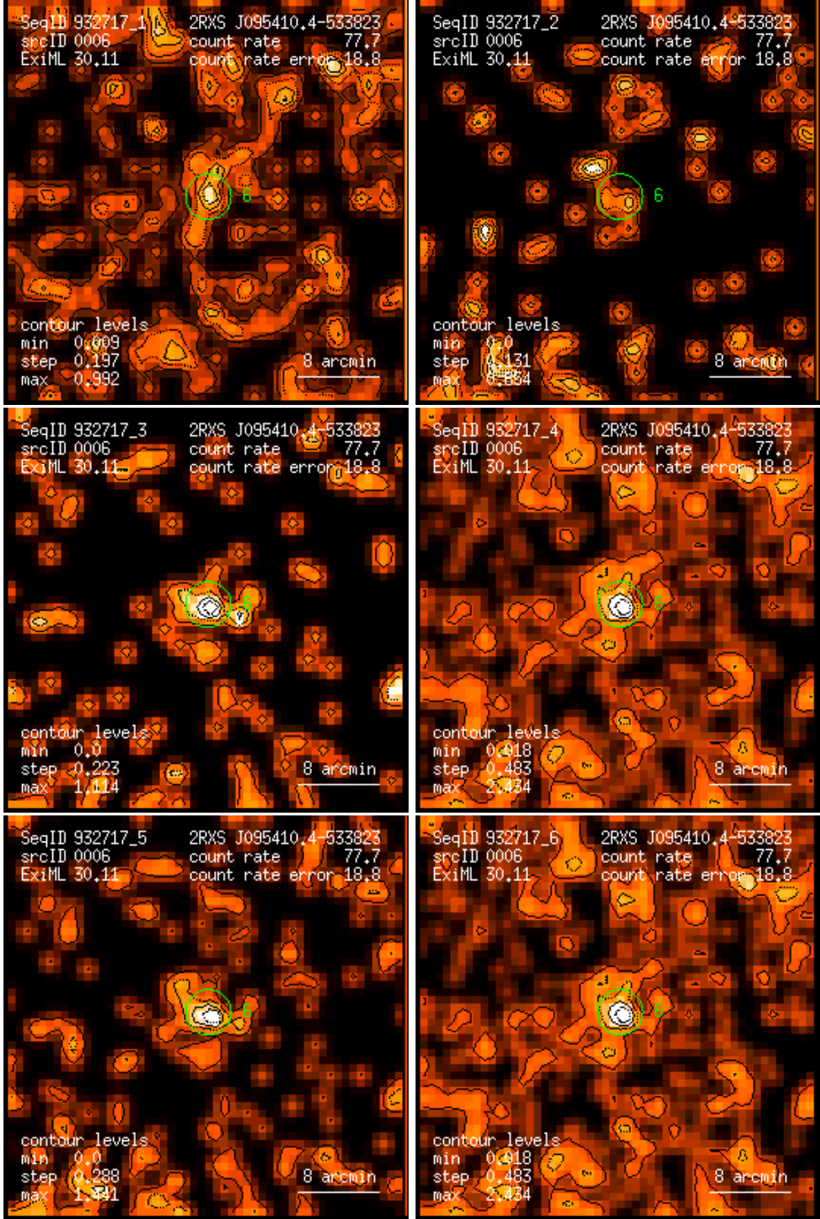
Figure 6: RASS 932717: detection 0006: band rate images, Gaussian filter: (1) PSPC channels 11 – 41, (2) 52 – 90, (3) 91 – 201, (4) 11 – 235, (5) 52 – 201, (6) 11 – 201. Broad band rates in counts/ks. Band rate contour levels in counts/ks/arcmin 2 .
