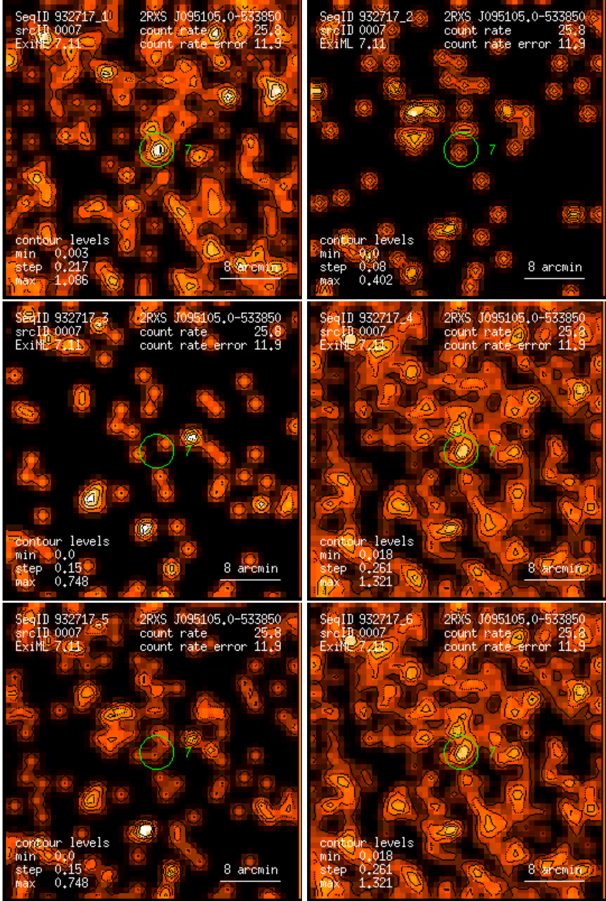
Figure 7: RASS 932717: detection 0007: band rate images, Gaussian filter: (1) PSPC channels 11 – 41, (2) 52 – 90, (3) 91 – 201, (4) 11 – 235, (5) 52 – 201, (6) 11 – 201. Broad band rates in counts/ks. Band rate contour levels in counts/ks/arcmin 2 .
