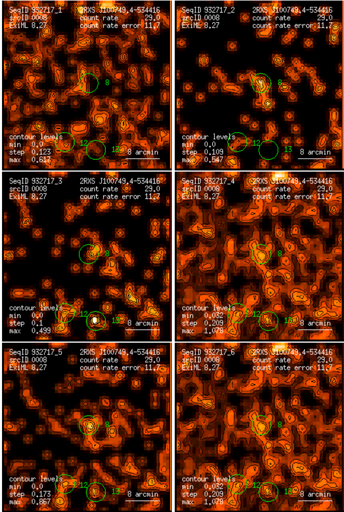
Figure 8: RASS 932717: detection 0008: band rate images, Gaussian filter: (1) PSPC channels 11 – 41, (2) 52 – 90, (3) 91 – 201, (4) 11 – 235, (5) 52 – 201, (6) 11 – 201. Broad band rates in counts/ks. Band rate contour levels in counts/ks/arcmin 2 .
