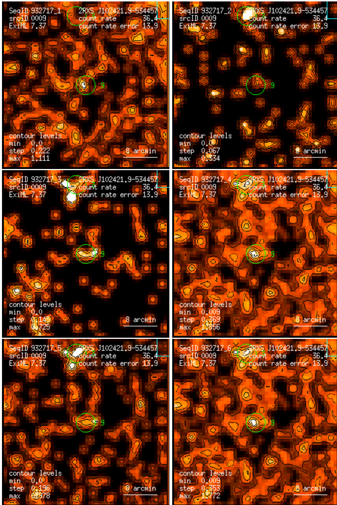
Figure 9: RASS 932717: detection 0009: band rate images, Gaussian filter: (1) PSPC channels 11 – 41, (2) 52 – 90, (3) 91 – 201, (4) 11 – 235, (5) 52 – 201, (6) 11 – 201. Broad band rates in counts/ks. Band rate contour levels in counts/ks/arcmin 2 .
