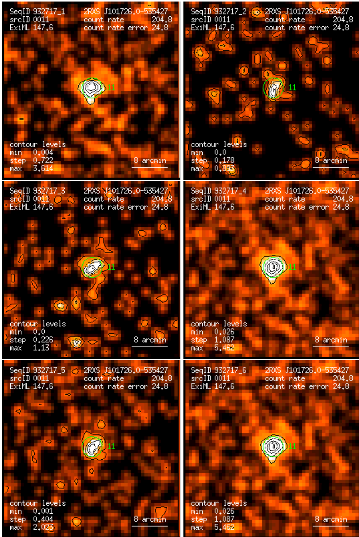
Figure 11: RASS 932717: detection 0011: band rate images, Gaussian filter: (1) PSPC channels 11 – 41, (2) 52 – 90, (3) 91 – 201, (4) 11 – 235, (5) 52 – 201, (6) 11 – 201. Broad band rates in counts/ks. Band rate contour levels in counts/ks/arcmin 2 .
