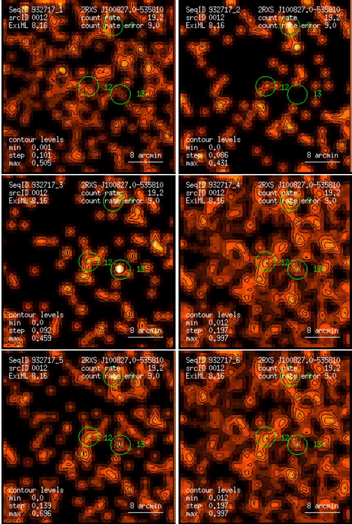
Figure 12: RASS 932717: detection 0012: band rate images, Gaussian filter: (1) PSPC channels 11 – 41, (2) 52 – 90, (3) 91 – 201, (4) 11 – 235, (5) 52 – 201, (6) 11 – 201. Broad band rates in counts/ks. Band rate contour levels in counts/ks/arcmin 2 .
