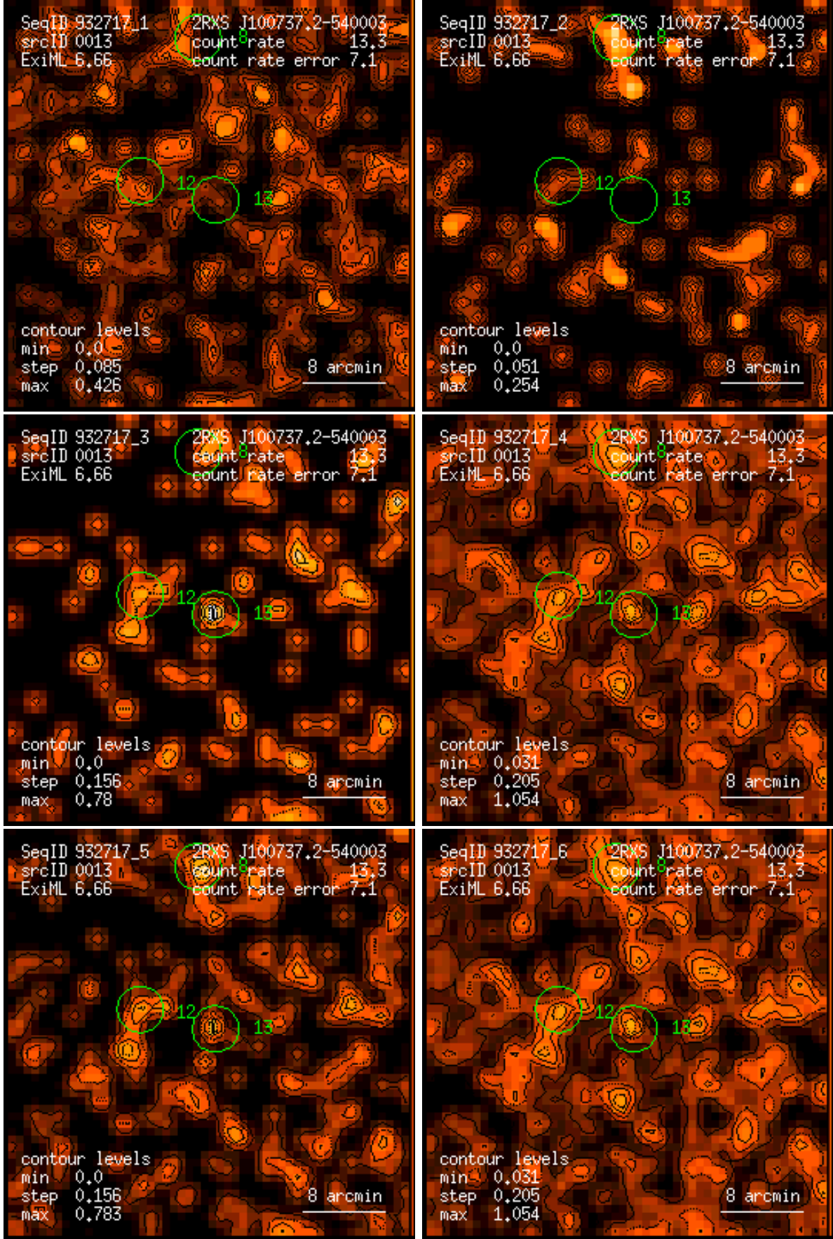
Figure 13: RASS 932717: detection 0013: band rate images, Gaussian filter: (1) PSPC channels 11 – 41, (2) 52 – 90, (3) 91 – 201, (4) 11 – 235, (5) 52 – 201, (6) 11 – 201. Broad band rates in counts/ks. Band rate contour levels in counts/ks/arcmin 2 .
