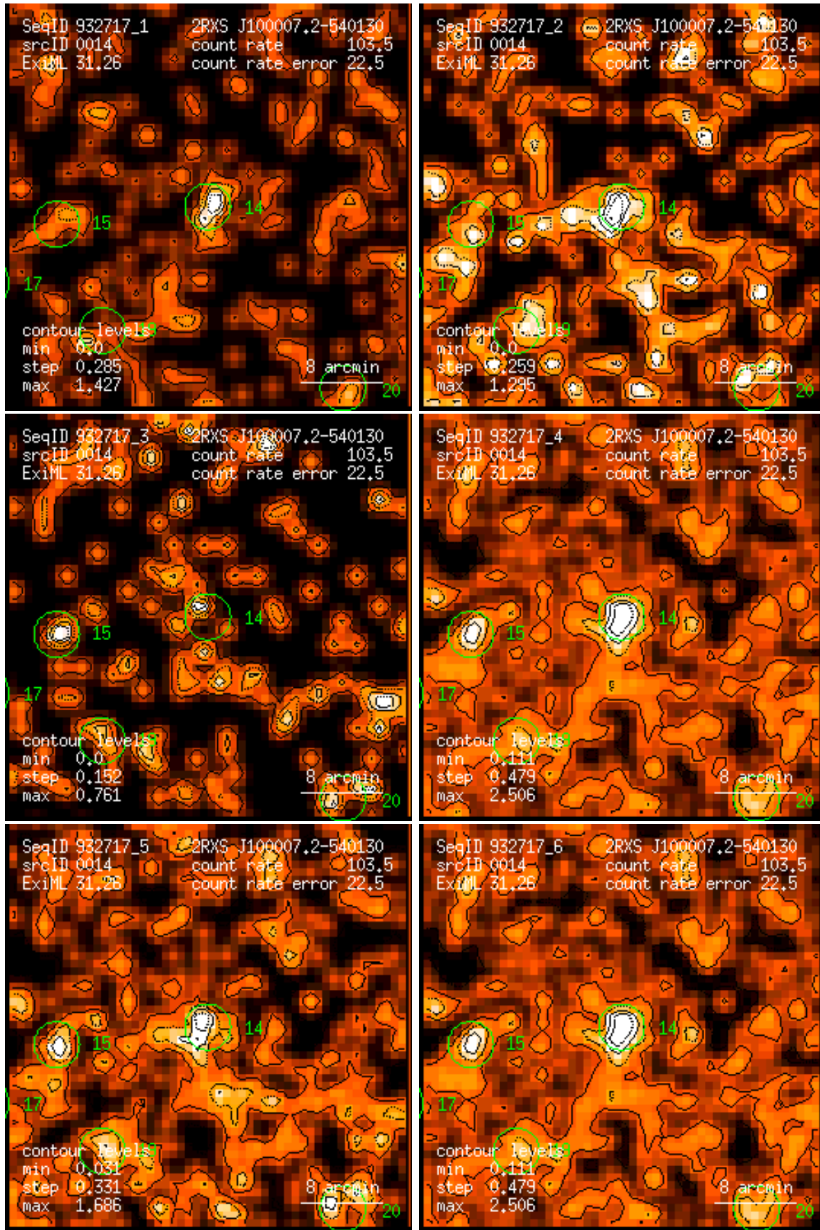
Figure 14: RASS 932717: detection 0014: band rate images, Gaussian filter: (1) PSPC channels 11 – 41, (2) 52 – 90, (3) 91 – 201, (4) 11 – 235, (5) 52 – 201, (6) 11 – 201. Broad band rates in counts/ks. Band rate contour levels in counts/ks/arcmin 2 .
