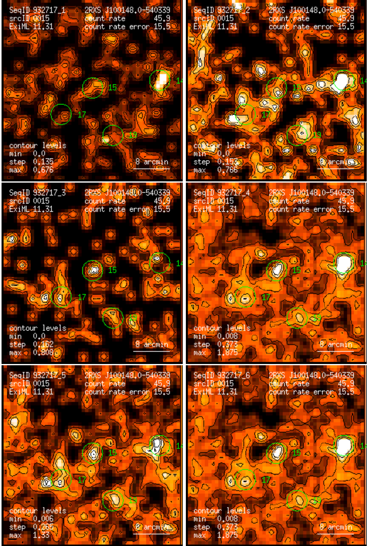
Figure 15: RASS 932717: detection 0015: band rate images, Gaussian filter: (1) PSPC channels 11 – 41, (2) 52 – 90, (3) 91 – 201, (4) 11 – 235, (5) 52 – 201, (6) 11 – 201. Broad band rates in counts/ks. Band rate contour levels in counts/ks/arcmin 2 .
