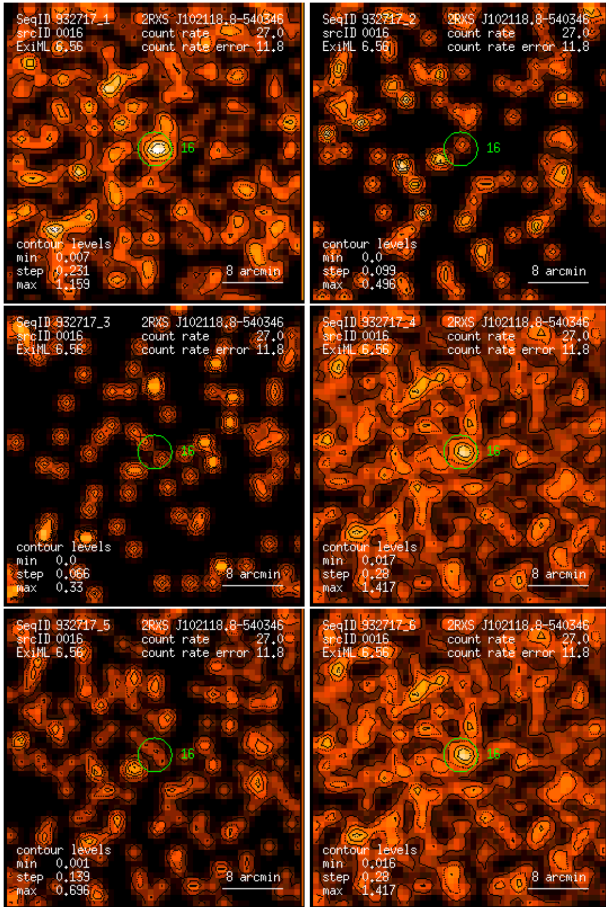
Figure 16: RASS 932717: detection 0016: band rate images, Gaussian filter: (1) PSPC channels 11 – 41, (2) 52 – 90, (3) 91 – 201, (4) 11 – 235, (5) 52 – 201, (6) 11 – 201. Broad band rates in counts/ks. Band rate contour levels in counts/ks/arcmin 2 .
