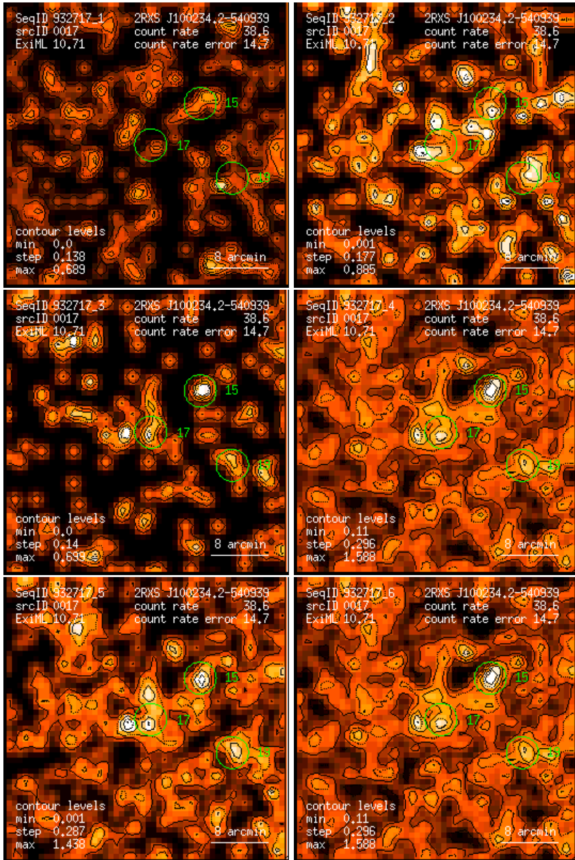
Figure 17: RASS 932717: detection 0017: band rate images, Gaussian filter: (1) PSPC channels 11 – 41, (2) 52 – 90, (3) 91 – 201, (4) 11 – 235, (5) 52 – 201, (6) 11 – 201. Broad band rates in counts/ks. Band rate contour levels in counts/ks/arcmin 2 .
