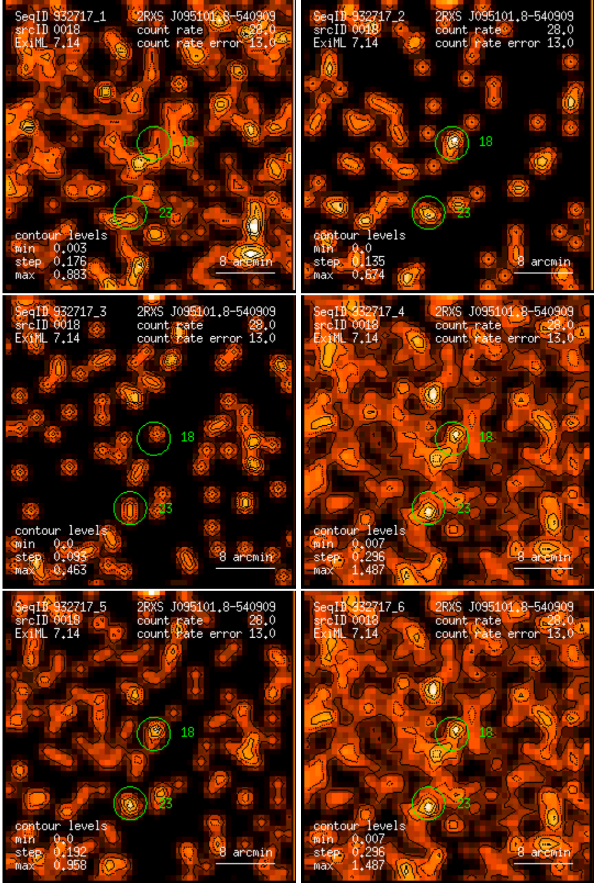
Figure 18: RASS 932717: detection 0018: band rate images, Gaussian filter: (1) PSPC channels 11 – 41, (2) 52 – 90, (3) 91 – 201, (4) 11 – 235, (5) 52 – 201, (6) 11 – 201. Broad band rates in counts/ks. Band rate contour levels in counts/ks/arcmin 2 .
