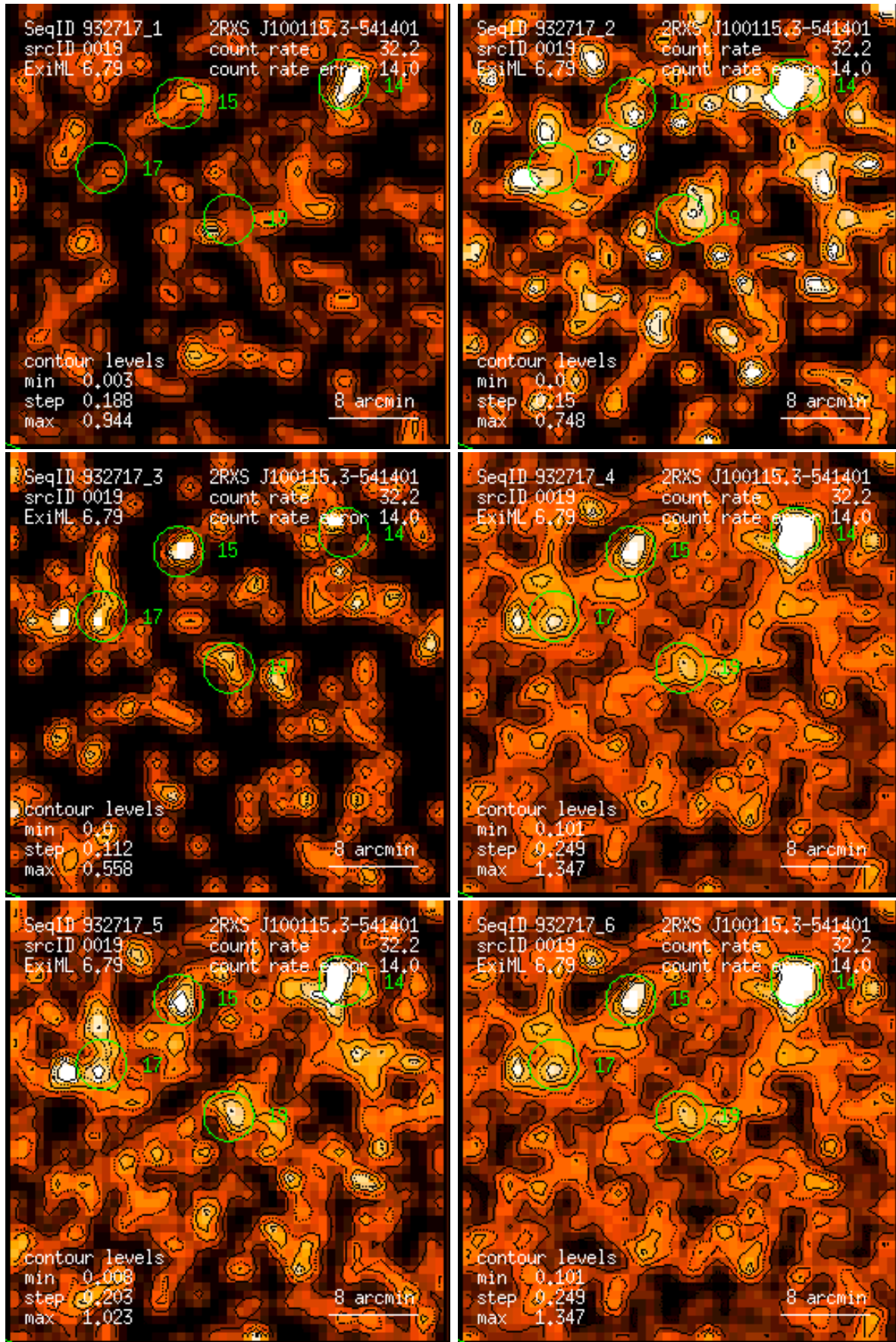
Figure 19: RASS 932717: detection 0019: band rate images, Gaussian filter: (1) PSPC channels 11 – 41, (2) 52 – 90, (3) 91 – 201, (4) 11 – 235, (5) 52 – 201, (6) 11 – 201. Broad band rates in counts/ks. Band rate contour levels in counts/ks/arcmin 2 .
