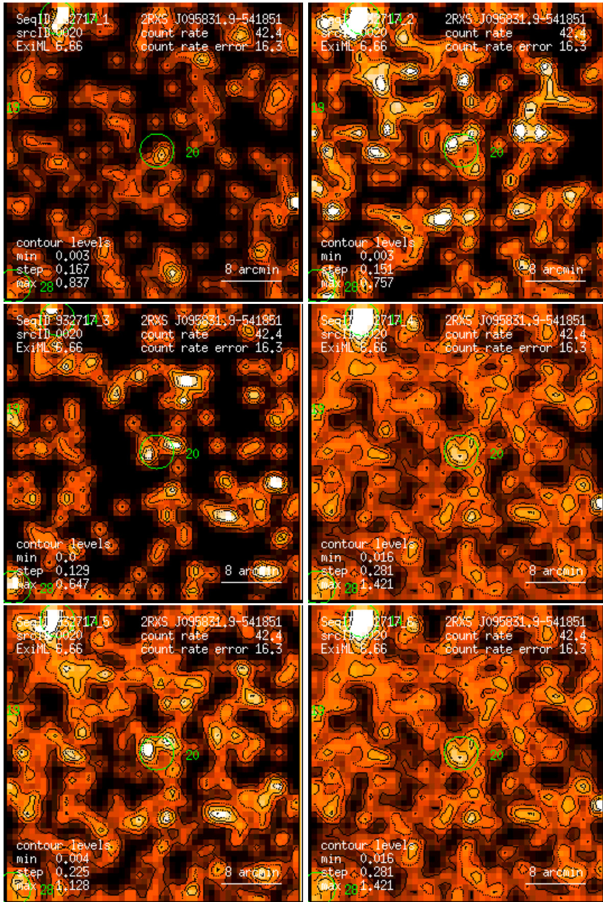
Figure 20: RASS 932717: detection 0020: band rate images, Gaussian filter: (1) PSPC channels 11 – 41, (2) 52 – 90, (3) 91 – 201, (4) 11 – 235, (5) 52 – 201, (6) 11 – 201. Broad band rates in counts/ks. Band rate contour levels in counts/ks/arcmin 2 .
