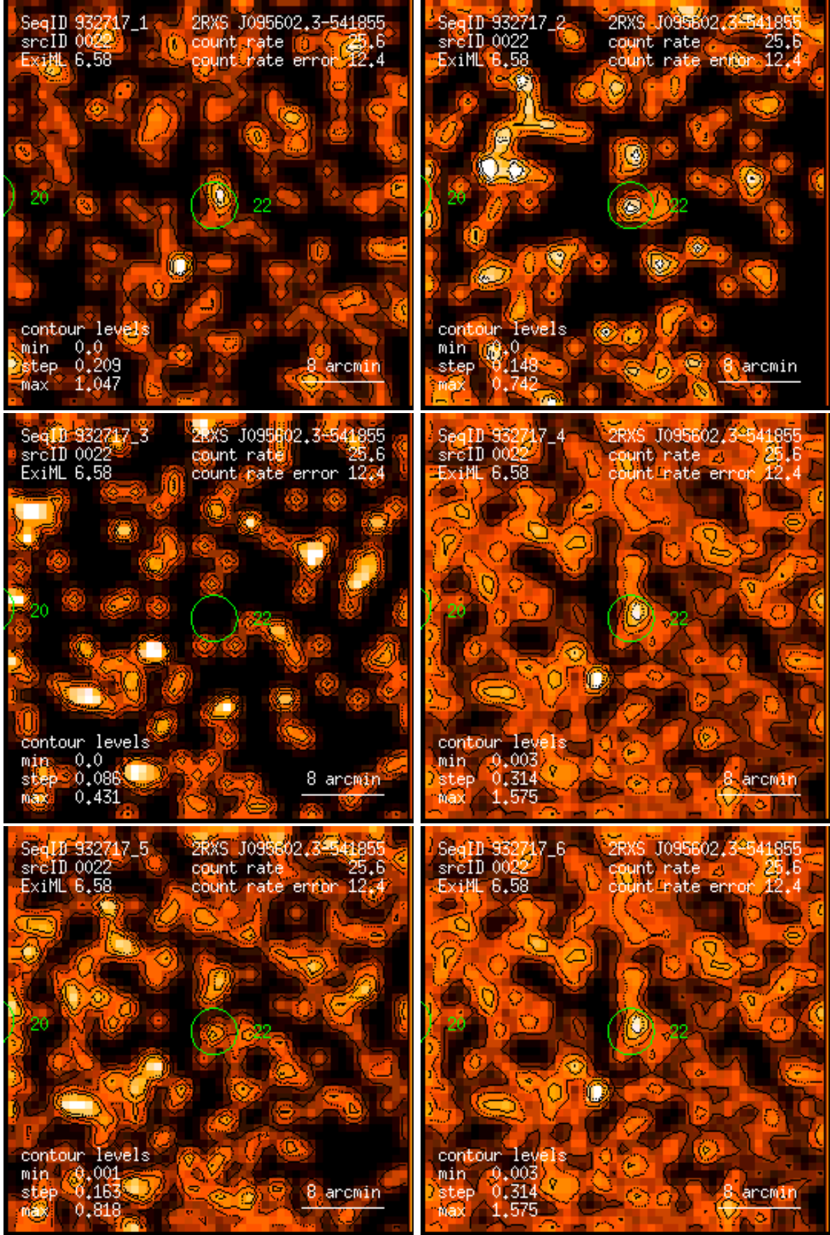
Figure 22: RASS 932717: detection 0022: band rate images, Gaussian filter: (1) PSPC channels 11 – 41, (2) 52 – 90, (3) 91 – 201, (4) 11 – 235, (5) 52 – 201, (6) 11 – 201. Broad band rates in counts/ks. Band rate contour levels in counts/ks/arcmin 2 .
