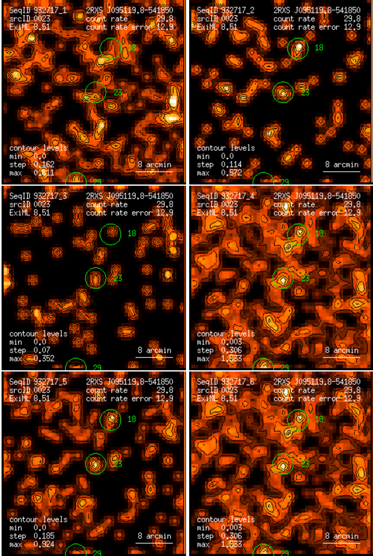
Figure 23: RASS 932717: detection 0023: band rate images, Gaussian filter: (1) PSPC channels 11 – 41, (2) 52 – 90, (3) 91 – 201, (4) 11 – 235, (5) 52 – 201, (6) 11 – 201. Broad band rates in counts/ks. Band rate contour levels in counts/ks/arcmin 2 .
