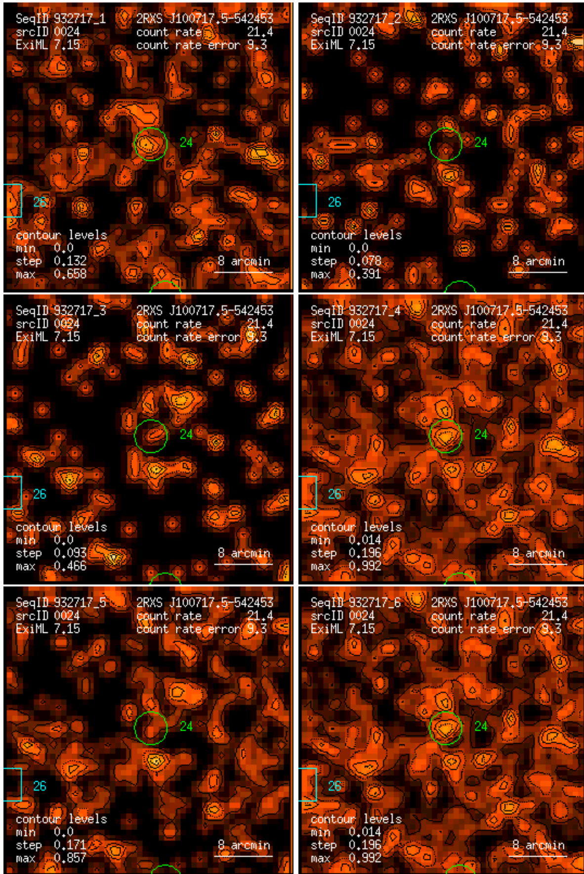
Figure 24: RASS 932717: detection 0024: band rate images, Gaussian filter: (1) PSPC channels 11 – 41, (2) 52 – 90, (3) 91 – 201, (4) 11 – 235, (5) 52 – 201, (6) 11 – 201. Broad band rates in counts/ks. Band rate contour levels in counts/ks/arcmin 2 .
