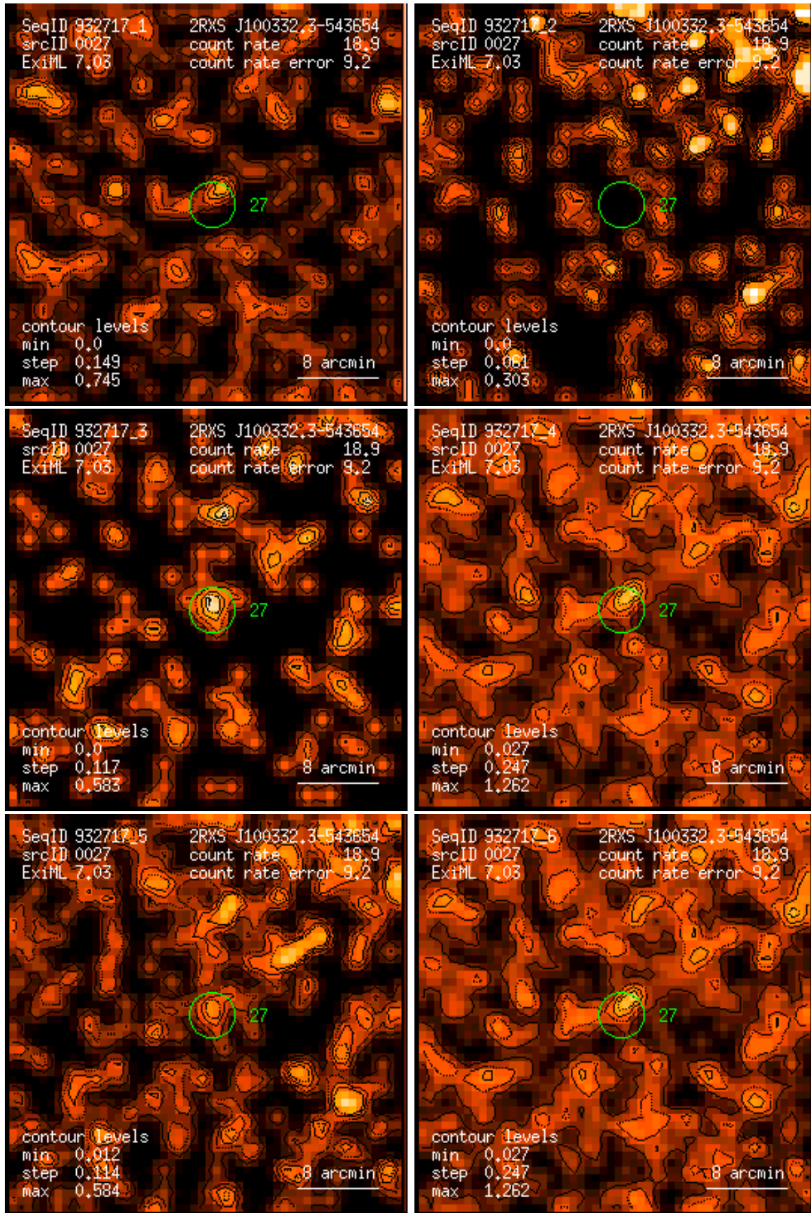
Figure 27: RASS 932717: detection 0027: band rate images, Gaussian filter: (1) PSPC channels 11 – 41, (2) 52 – 90, (3) 91 – 201, (4) 11 – 235, (5) 52 – 201, (6) 11 – 201. Broad band rates in counts/ks. Band rate contour levels in counts/ks/arcmin 2 .
