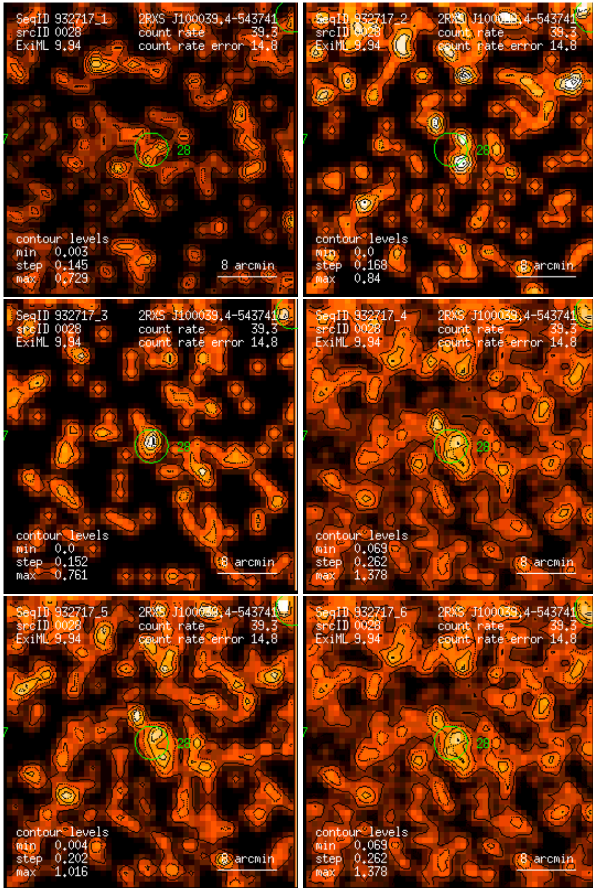
Figure 28: RASS 932717: detection 0028: band rate images, Gaussian filter: (1) PSPC channels 11 – 41, (2) 52 – 90, (3) 91 – 201, (4) 11 – 235, (5) 52 – 201, (6) 11 – 201. Broad band rates in counts/ks. Band rate contour levels in counts/ks/arcmin 2 .
