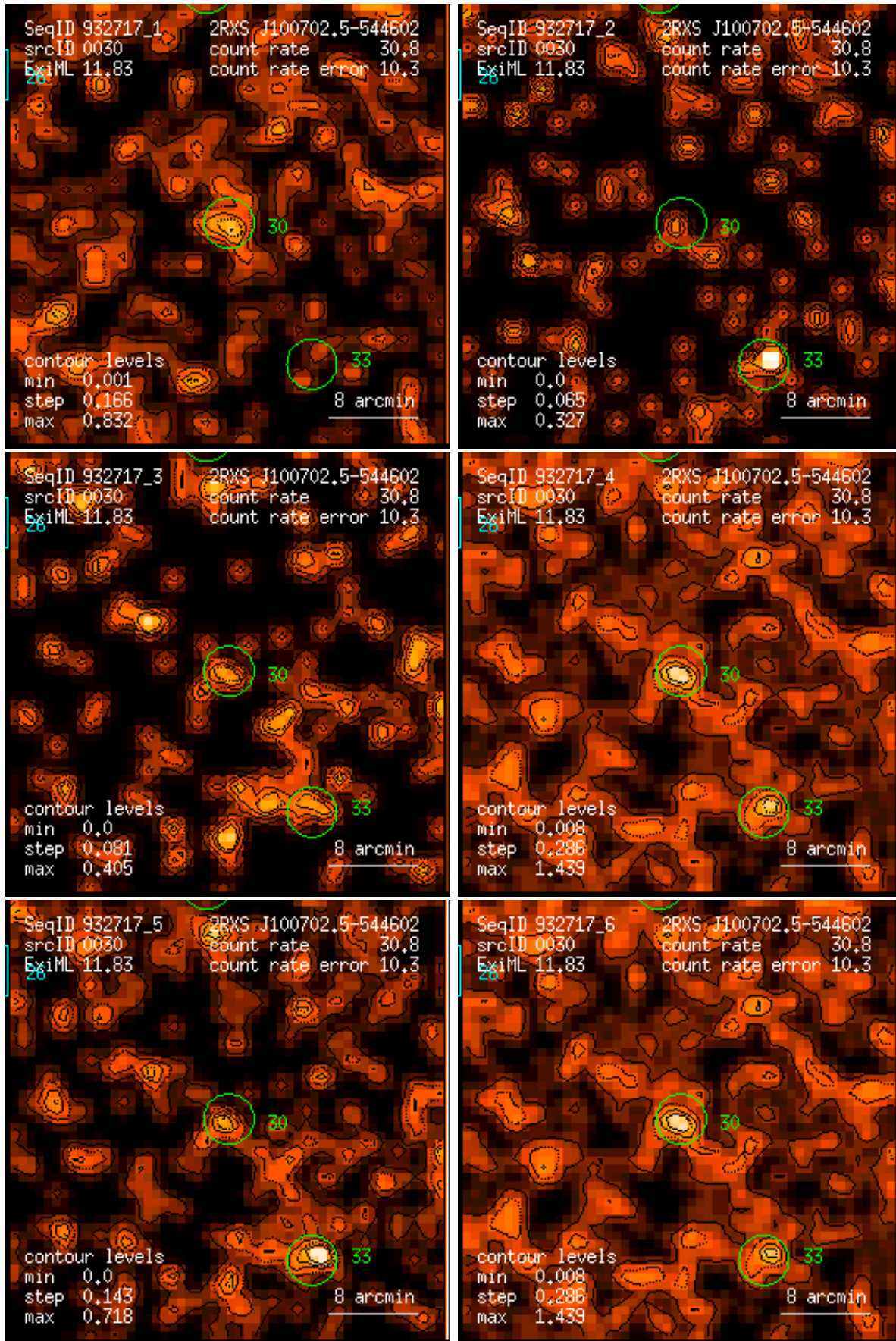
Figure 30: RASS 932717: detection 0030: band rate images, Gaussian filter: (1) PSPC channels 11 – 41, (2) 52 – 90, (3) 91 – 201, (4) 11 – 235, (5) 52 – 201, (6) 11 – 201. Broad band rates in counts/ks. Band rate contour levels in counts/ks/arcmin 2 .
