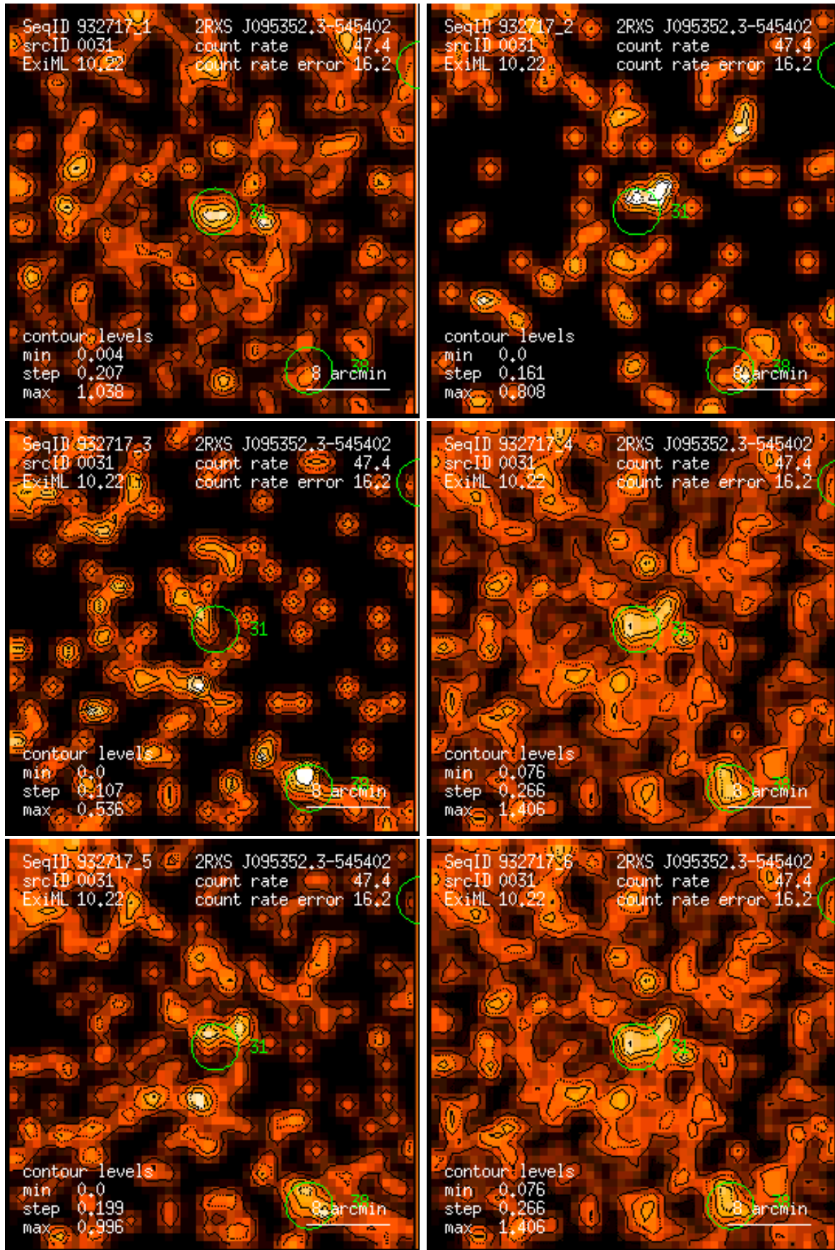
Figure 31: RASS 932717: detection 0031: band rate images, Gaussian filter: (1) PSPC channels 11 – 41, (2) 52 – 90, (3) 91 – 201, (4) 11 – 235, (5) 52 – 201, (6) 11 – 201. Broad band rates in counts/ks. Band rate contour levels in counts/ks/arcmin 2 .
