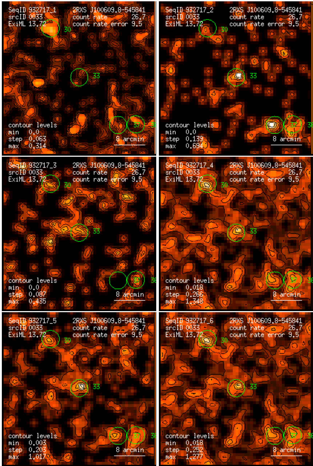
Figure 33: RASS 932717: detection 0033: band rate images, Gaussian filter: (1) PSPC channels 11 – 41, (2) 52 – 90, (3) 91 – 201, (4) 11 – 235, (5) 52 – 201, (6) 11 – 201. Broad band rates in counts/ks. Band rate contour levels in counts/ks/arcmin 2 .
