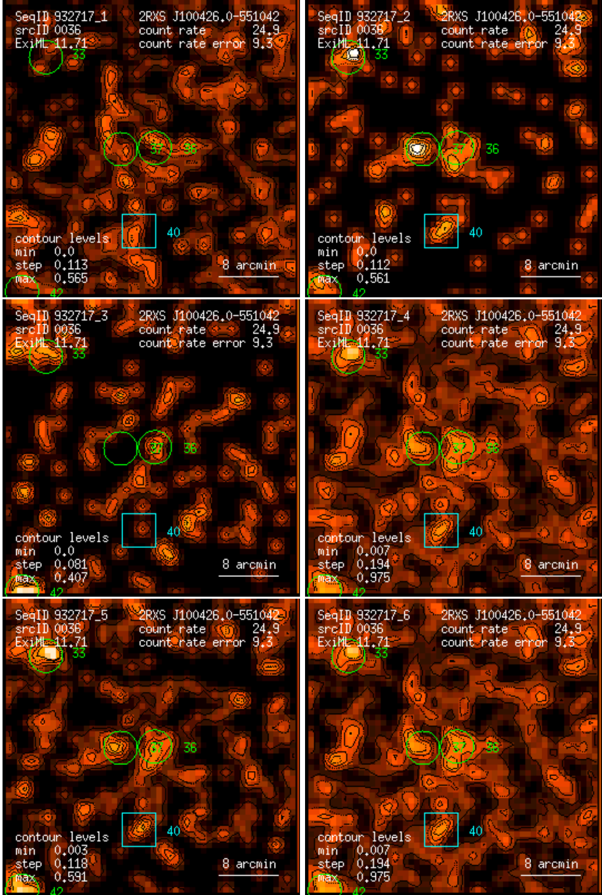
Figure 36: RASS 932717: detection 0036: band rate images, Gaussian filter: (1) PSPC channels 11 – 41, (2) 52 – 90, (3) 91 – 201, (4) 11 – 235, (5) 52 – 201, (6) 11 – 201. Broad band rates in counts/ks. Band rate contour levels in counts/ks/arcmin 2 .
