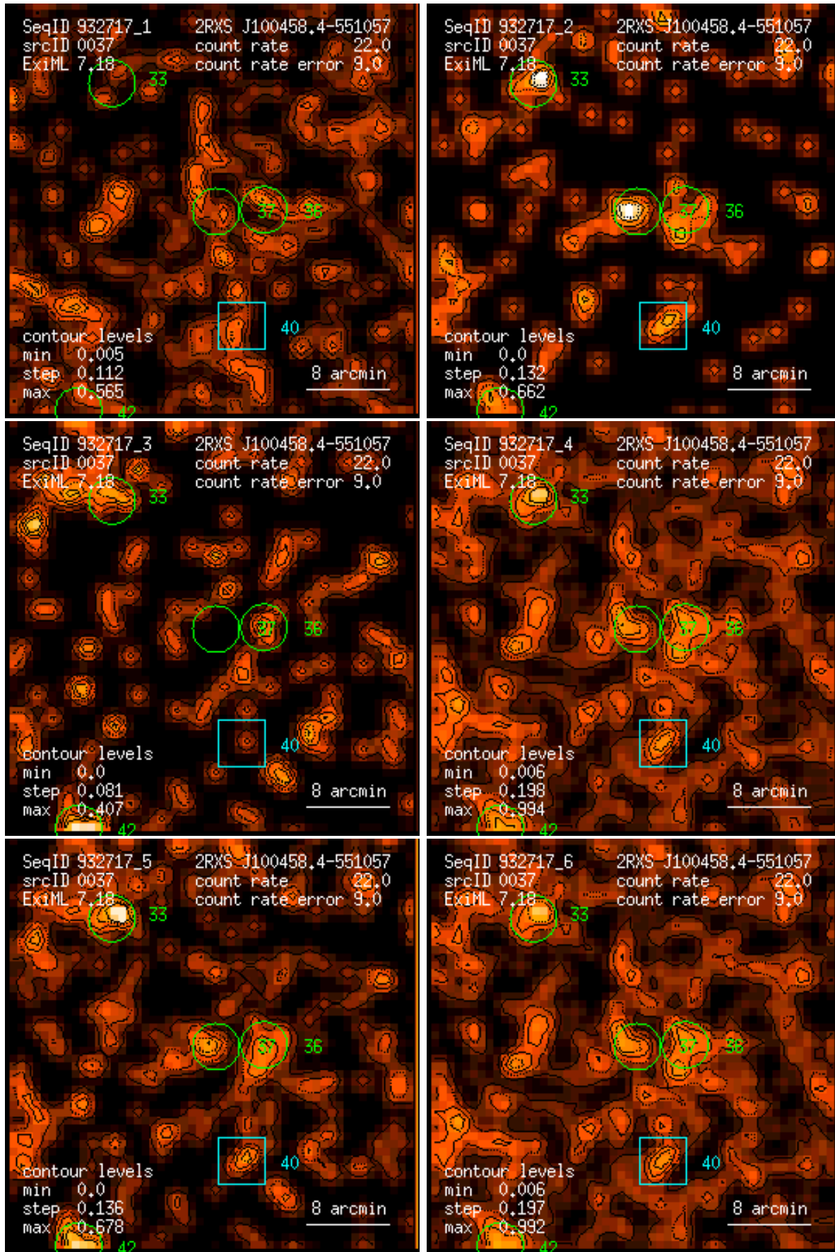
Figure 37: RASS 932717: detection 0037: band rate images, Gaussian filter: (1) PSPC channels 11 – 41, (2) 52 – 90, (3) 91 – 201, (4) 11 – 235, (5) 52 – 201, (6) 11 – 201. Broad band rates in counts/ks. Band rate contour levels in counts/ks/arcmin 2 .
