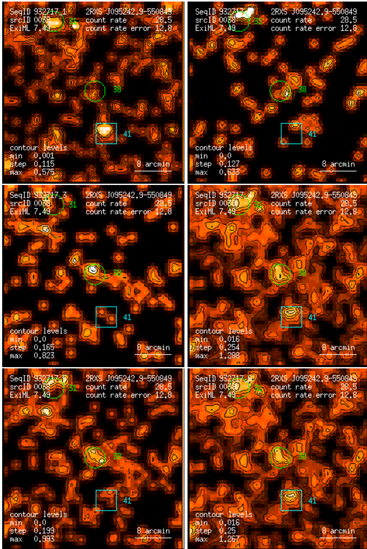
Figure 38: RASS 932717: detection 0038: band rate images, Gaussian filter: (1) PSPC channels 11 – 41, (2) 52 – 90, (3) 91 – 201, (4) 11 – 235, (5) 52 – 201, (6) 11 – 201. Broad band rates in counts/ks. Band rate contour levels in counts/ks/arcmin 2 .
