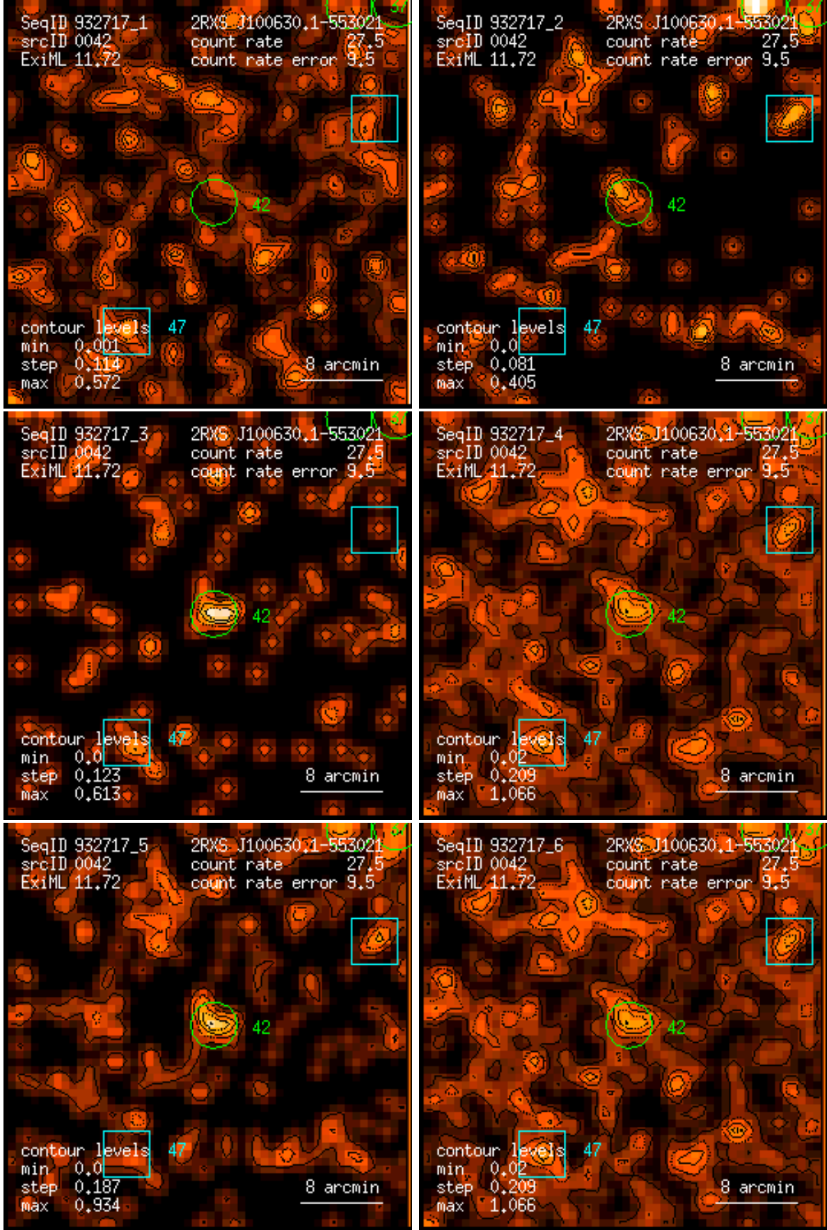
Figure 42: RASS 932717: detection 0042: band rate images, Gaussian filter: (1) PSPC channels 11 – 41, (2) 52 – 90, (3) 91 – 201, (4) 11 – 235, (5) 52 – 201, (6) 11 – 201. Broad band rates in counts/ks. Band rate contour levels in counts/ks/arcmin 2 .
