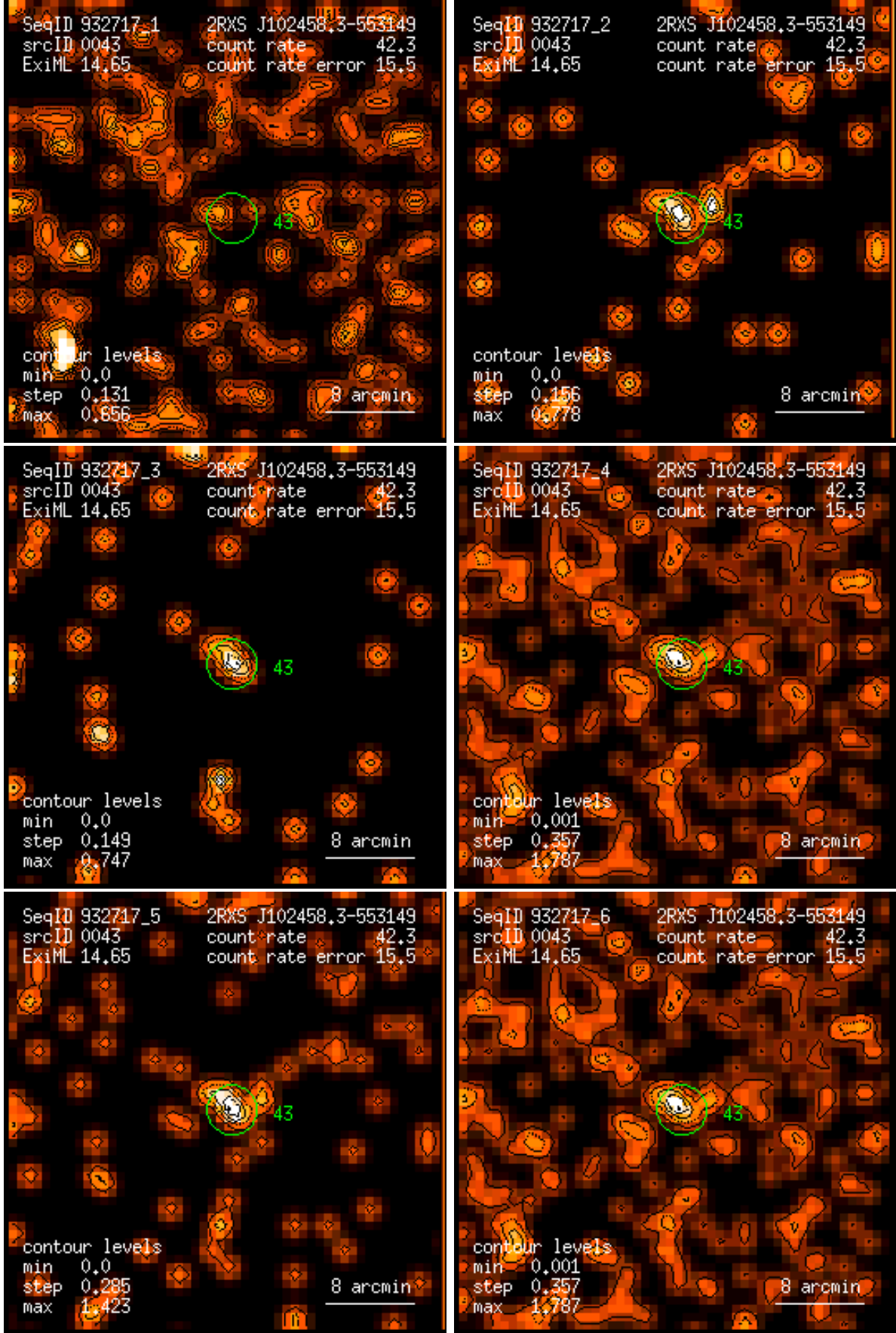
Figure 43: RASS 932717: detection 0043: band rate images, Gaussian filter: (1) PSPC channels 11 – 41, (2) 52 – 90, (3) 91 – 201, (4) 11 – 235, (5) 52 – 201, (6) 11 – 201. Broad band rates in counts/ks. Band rate contour levels in counts/ks/arcmin 2 .
