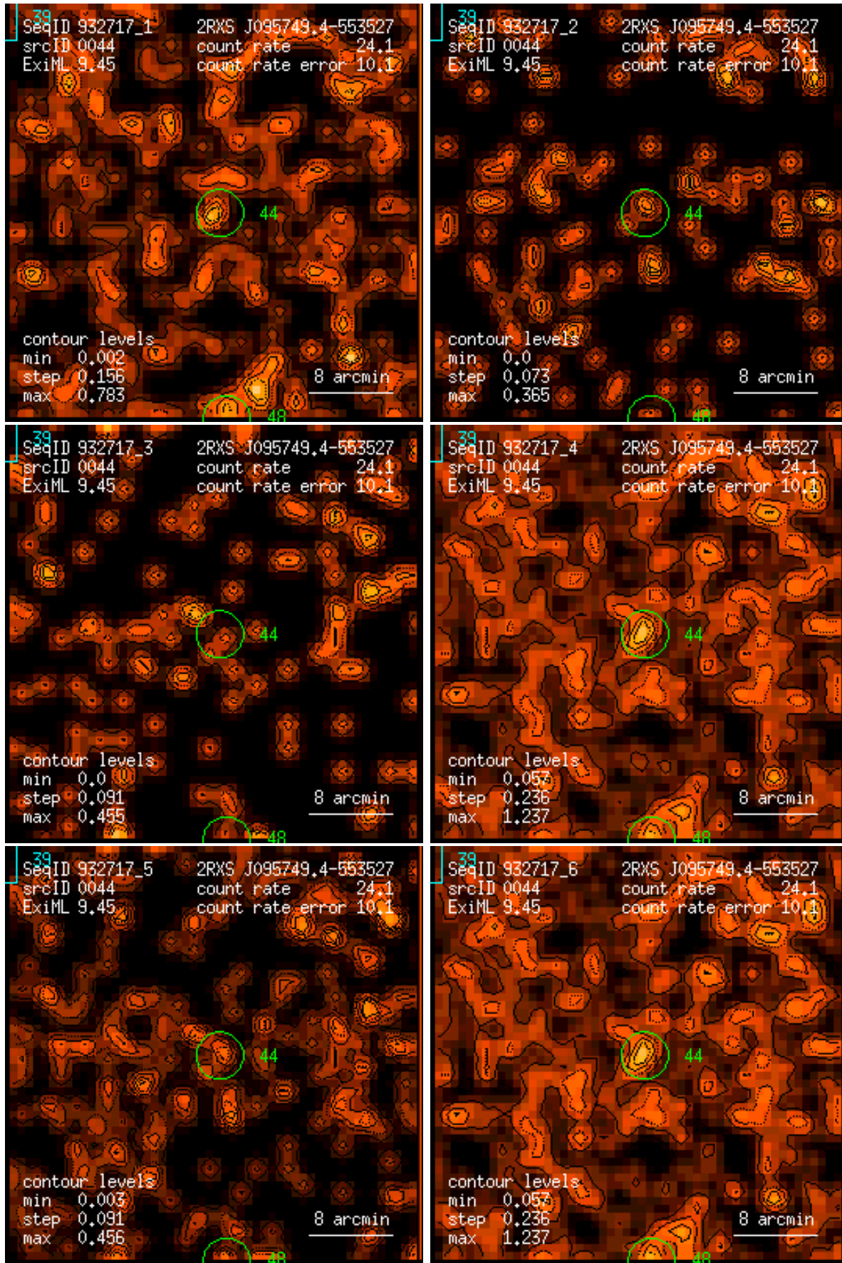
Figure 44: RASS 932717: detection 0044: band rate images, Gaussian filter: (1) PSPC channels 11 – 41, (2) 52 – 90, (3) 91 – 201, (4) 11 – 235, (5) 52 – 201, (6) 11 – 201. Broad band rates in counts/ks. Band rate contour levels in counts/ks/arcmin 2 .
