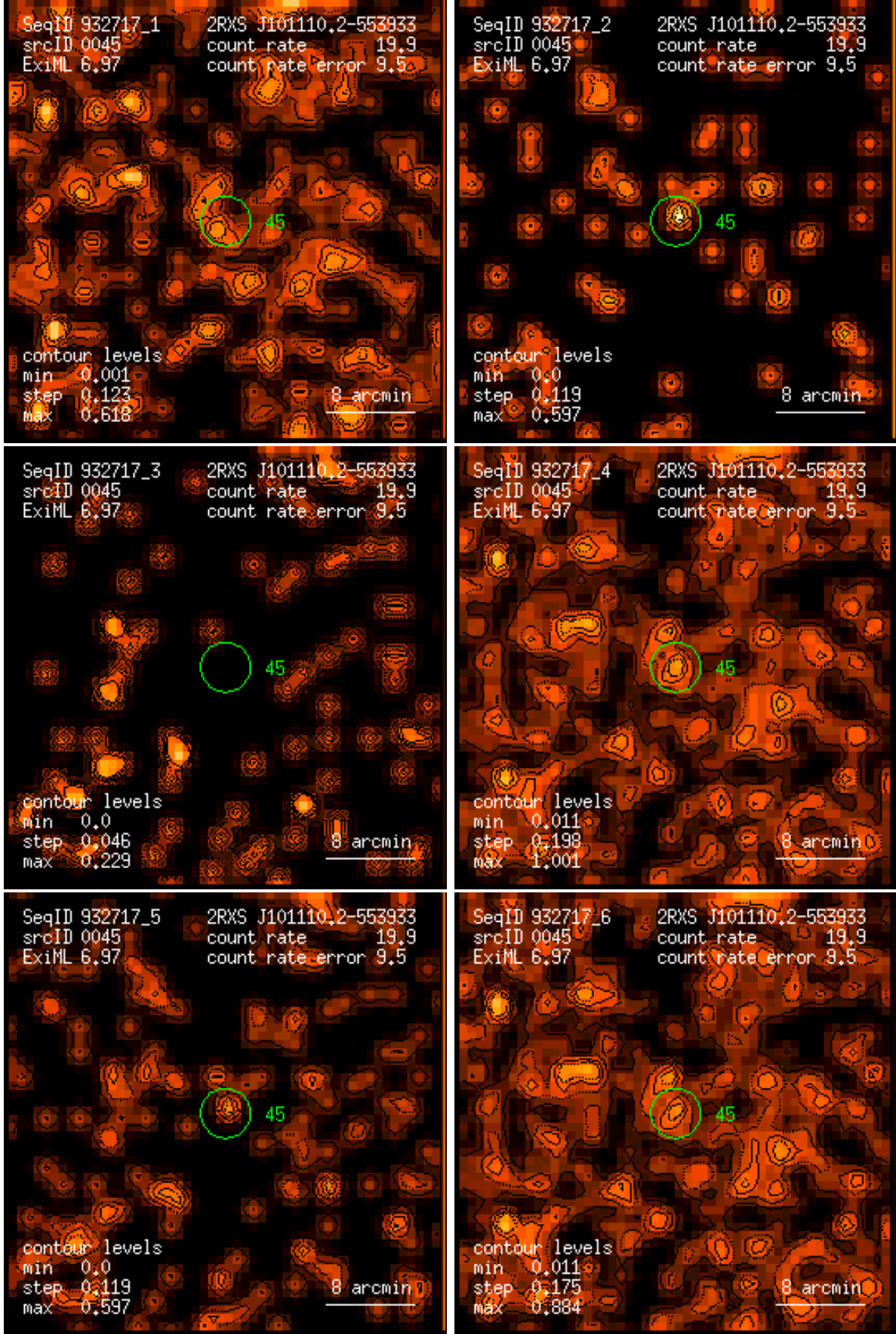
Figure 45: RASS 932717: detection 0045: band rate images, Gaussian filter: (1) PSPC channels 11 – 41, (2) 52 – 90, (3) 91 – 201, (4) 11 – 235, (5) 52 – 201, (6) 11 – 201. Broad band rates in counts/ks. Band rate contour levels in counts/ks/arcmin 2 .
