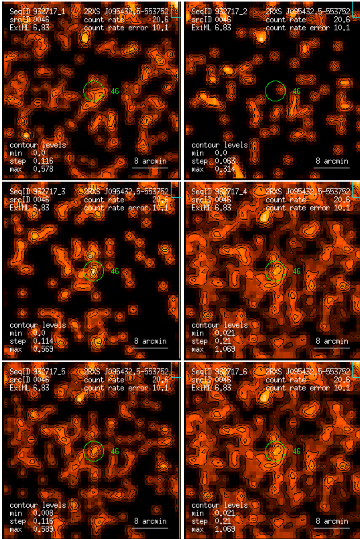
Figure 46: RASS 932717: detection 0046: band rate images, Gaussian filter: (1) PSPC channels 11 – 41, (2) 52 – 90, (3) 91 – 201, (4) 11 – 235, (5) 52 – 201, (6) 11 – 201. Broad band rates in counts/ks. Band rate contour levels in counts/ks/arcmin 2 .
