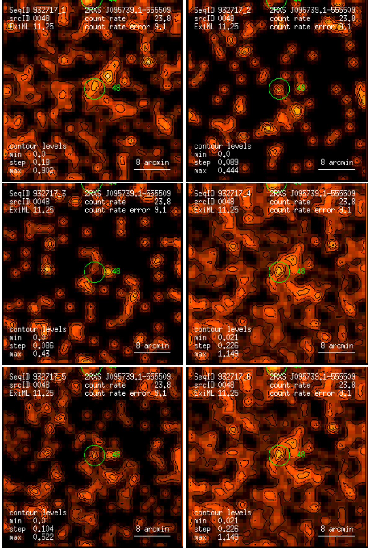
Figure 48: RASS 932717: detection 0048: band rate images, Gaussian filter: (1) PSPC channels 11 – 41, (2) 52 – 90, (3) 91 – 201, (4) 11 – 235, (5) 52 – 201, (6) 11 – 201. Broad band rates in counts/ks. Band rate contour levels in counts/ks/arcmin 2 .
