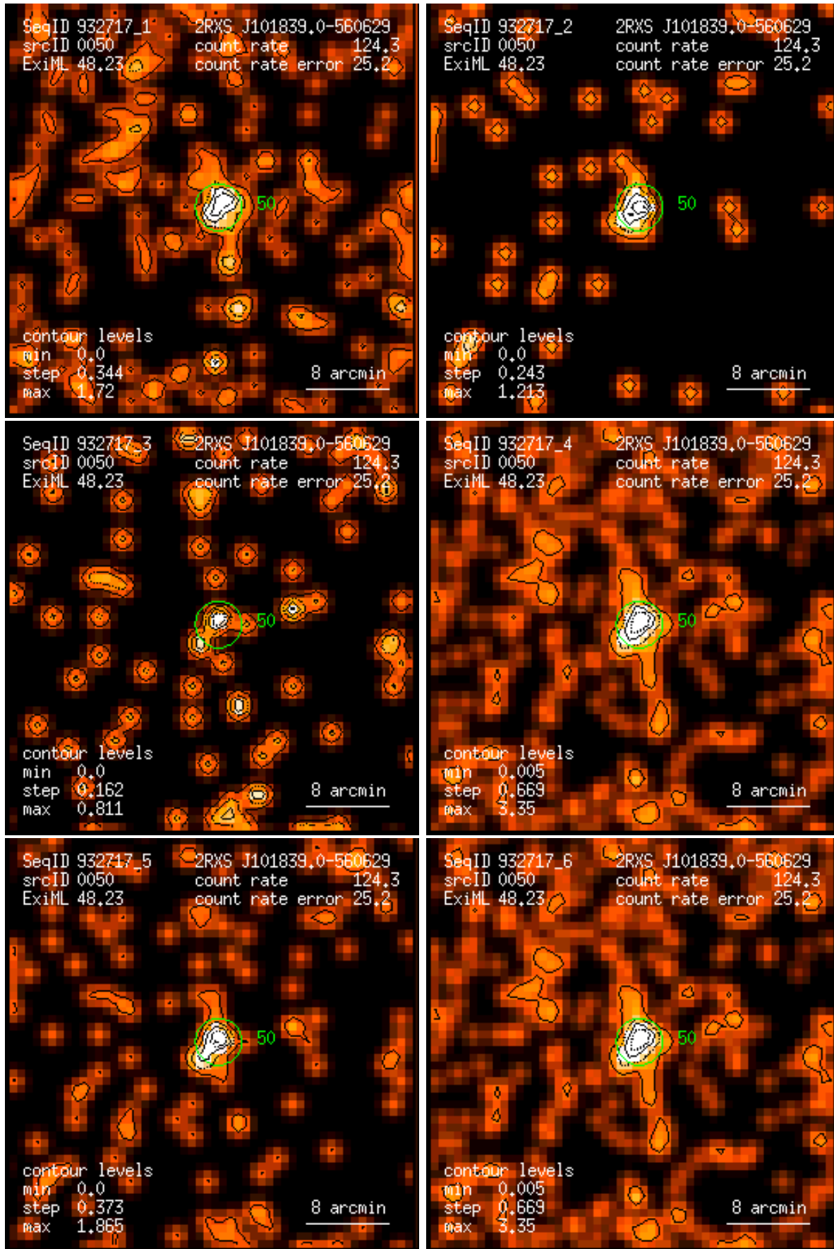
Figure 50: RASS 932717: detection 0050: band rate images, Gaussian filter: (1) PSPC channels 11 – 41, (2) 52 – 90, (3) 91 – 201, (4) 11 – 235, (5) 52 – 201, (6) 11 – 201. Broad band rates in counts/ks. Band rate contour levels in counts/ks/arcmin 2 .
