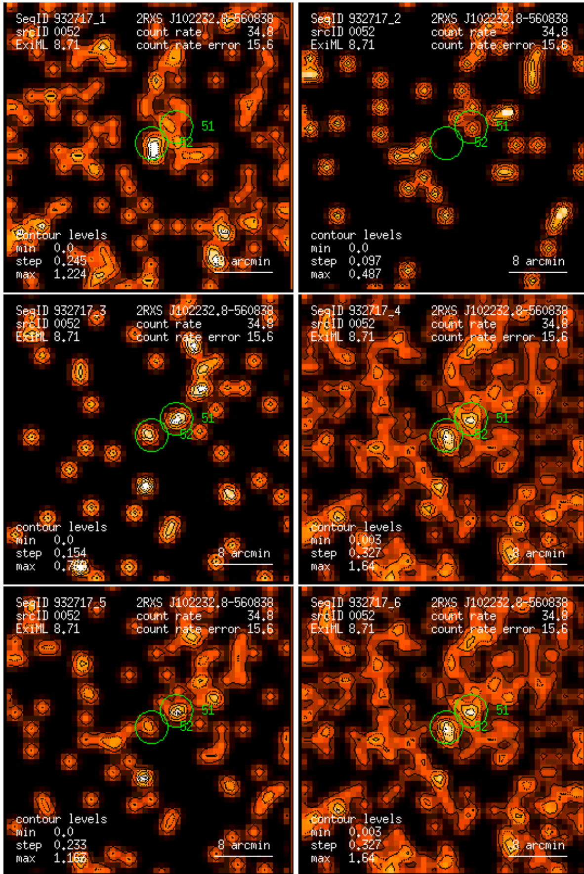
Figure 52: RASS 932717: detection 0052: band rate images, Gaussian filter: (1) PSPC channels 11 – 41, (2) 52 – 90, (3) 91 – 201, (4) 11 – 235, (5) 52 – 201, (6) 11 – 201. Broad band rates in counts/ks. Band rate contour levels in counts/ks/arcmin 2 .
