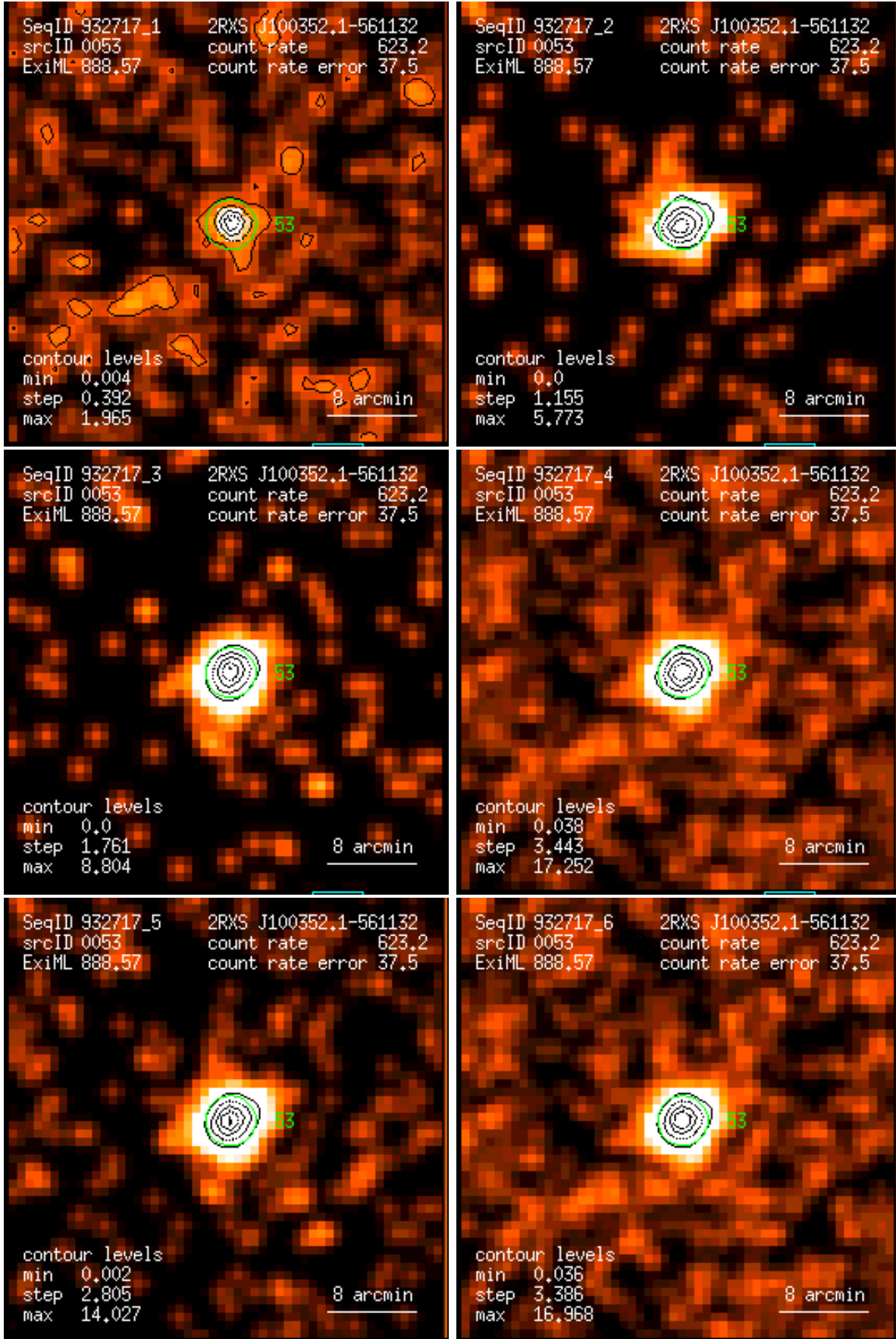
Figure 53: RASS 932717: detection 0053: band rate images, Gaussian filter: (1) PSPC channels 11 – 41, (2) 52 – 90, (3) 91 – 201, (4) 11 – 235, (5) 52 – 201, (6) 11 – 201. Broad band rates in counts/ks. Band rate contour levels in counts/ks/arcmin 2 .
