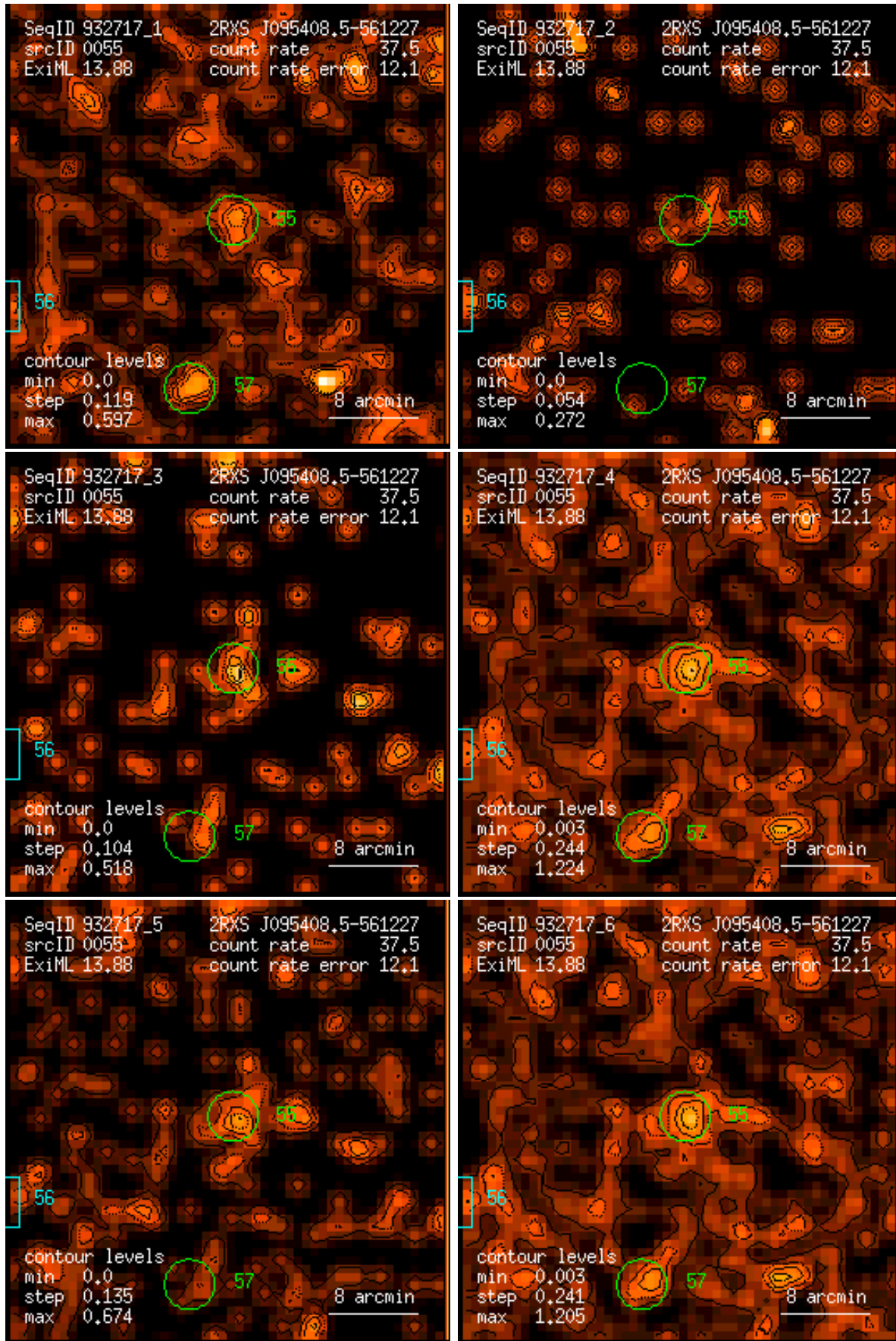
Figure 55: RASS 932717: detection 0055: band rate images, Gaussian filter: (1) PSPC channels 11 – 41, (2) 52 – 90, (3) 91 – 201, (4) 11 – 235, (5) 52 – 201, (6) 11 – 201. Broad band rates in counts/ks. Band rate contour levels in counts/ks/arcmin 2 .
