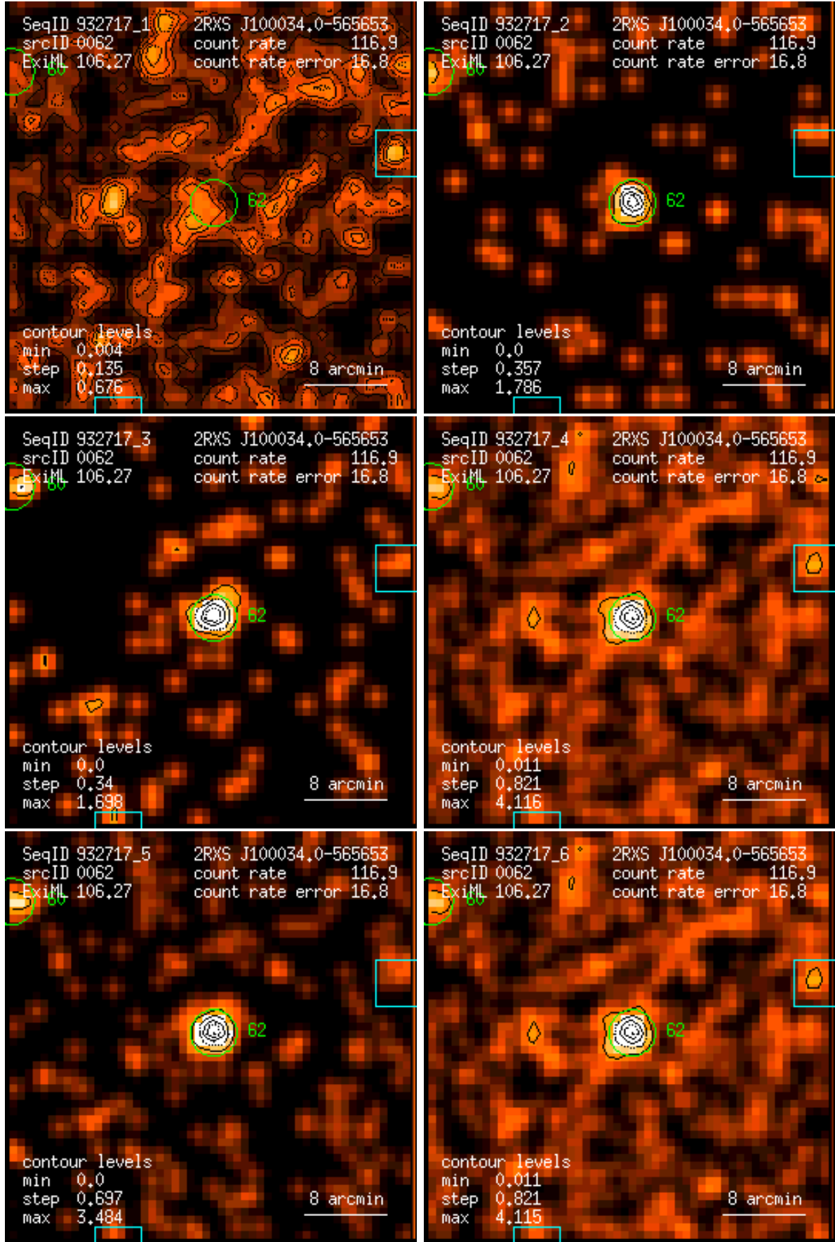
Figure 62: RASS 932717: detection 0062: band rate images, Gaussian filter: (1) PSPC channels 11 – 41, (2) 52 – 90, (3) 91 – 201, (4) 11 – 235, (5) 52 – 201, (6) 11 – 201. Broad band rates in counts/ks. Band rate contour levels in counts/ks/arcmin 2 .
