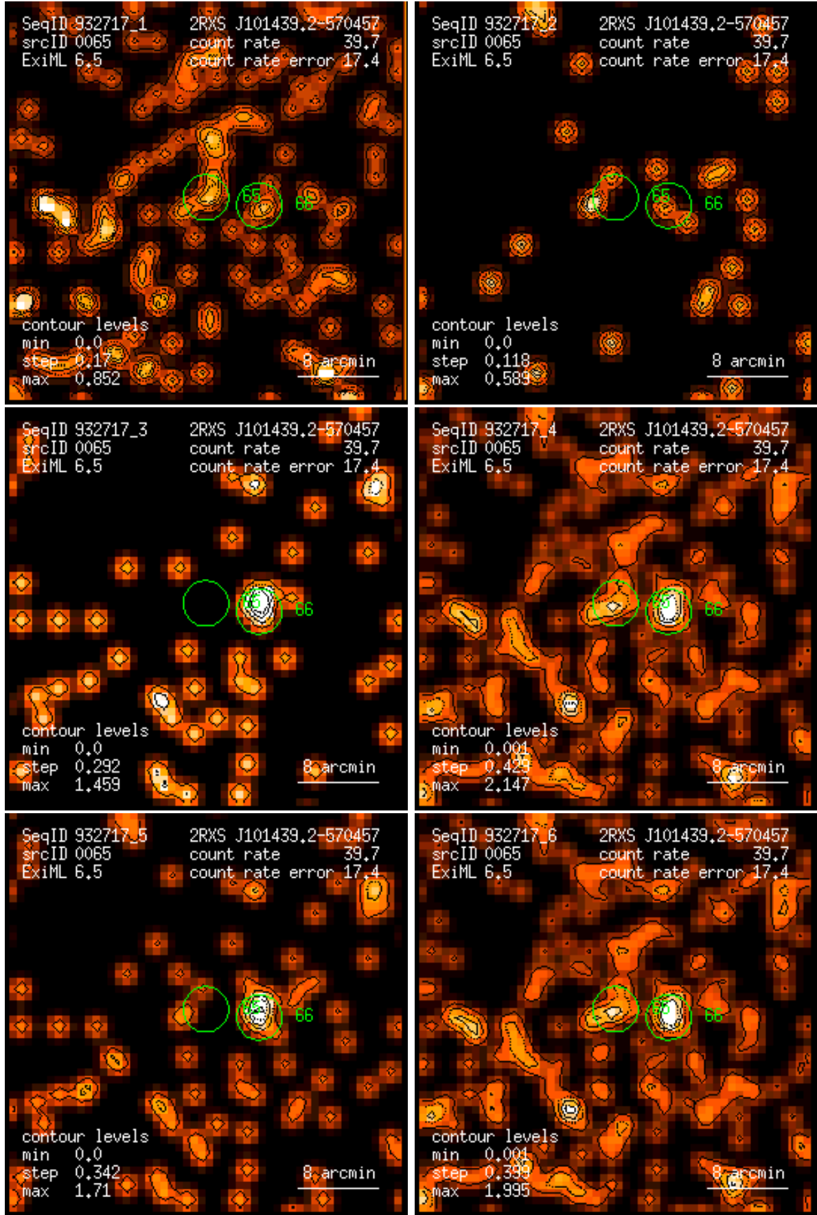
Figure 65: RASS 932717: detection 0065: band rate images, Gaussian filter: (1) PSPC channels 11 – 41, (2) 52 – 90, (3) 91 – 201, (4) 11 – 235, (5) 52 – 201, (6) 11 – 201. Broad band rates in counts/ks. Band rate contour levels in counts/ks/arcmin 2 .
