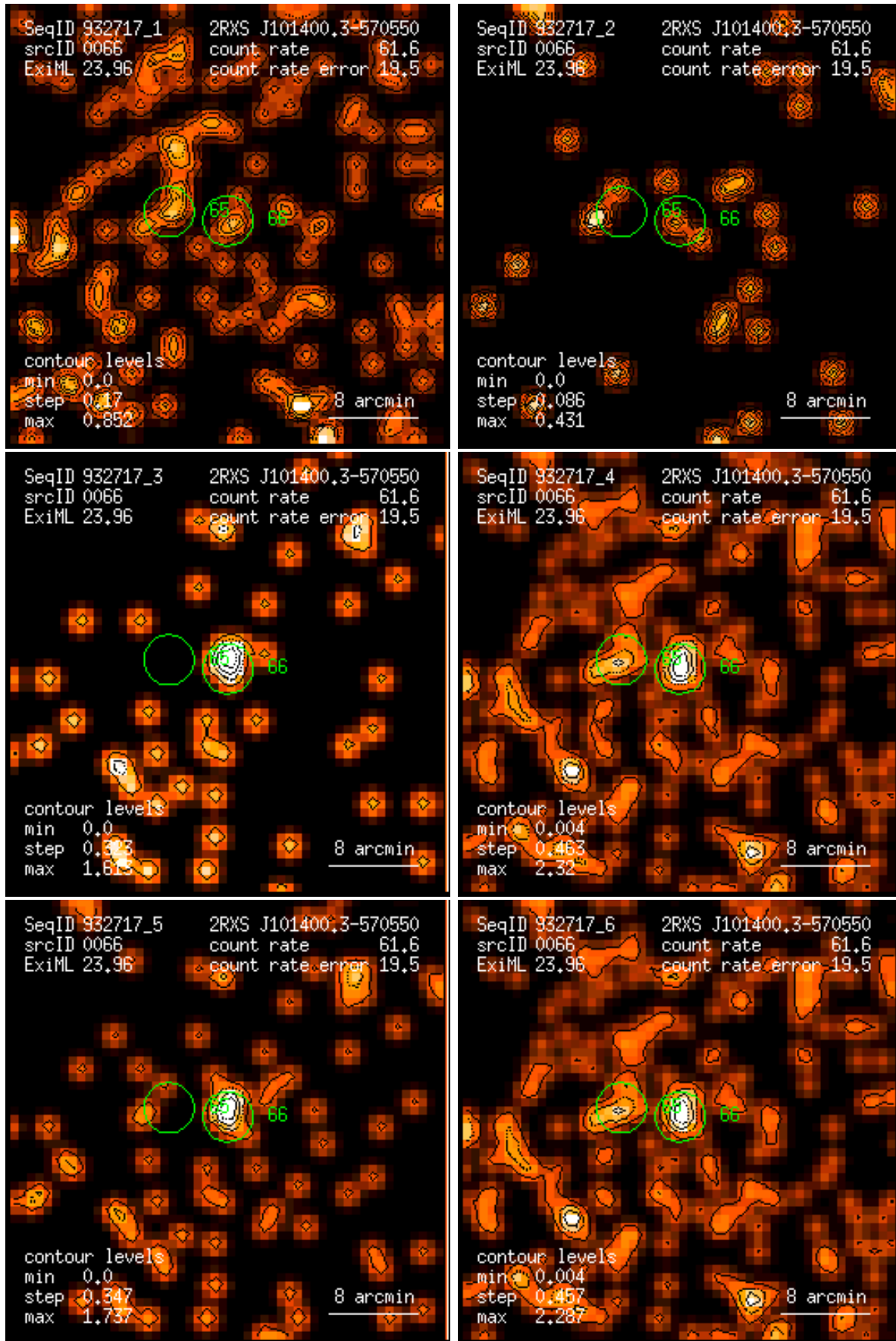
Figure 66: RASS 932717: detection 0066: band rate images, Gaussian filter: (1) PSPC channels 11 – 41, (2) 52 – 90, (3) 91 – 201, (4) 11 – 235, (5) 52 – 201, (6) 11 – 201. Broad band rates in counts/ks. Band rate contour levels in counts/ks/arcmin 2 .
